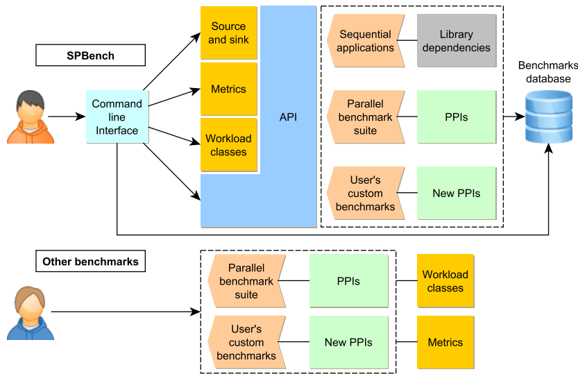
Fig. 1: SPBENCH methodology versus other benchmarks.
