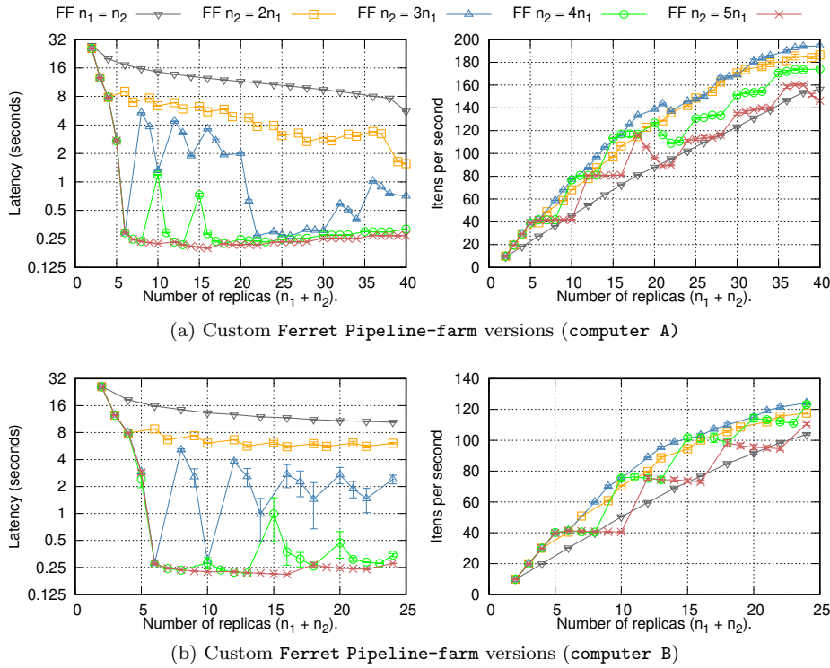
Fig. 7: Latency and throughput for the custom pipe-farm versions of Ferret. These versions are defined as pipe(seq(source), farm((seg,ext,vect), n_1 ), farm(rank, n_2 ), seq(sink)) , where n_1 and n_2 are the number of workers. The five versions represent different proportions of the number of workers in each Farm. E.g., n_2 = 3n_1 means that every time n_2 is increased by 3, n_1 is increased by 1.
