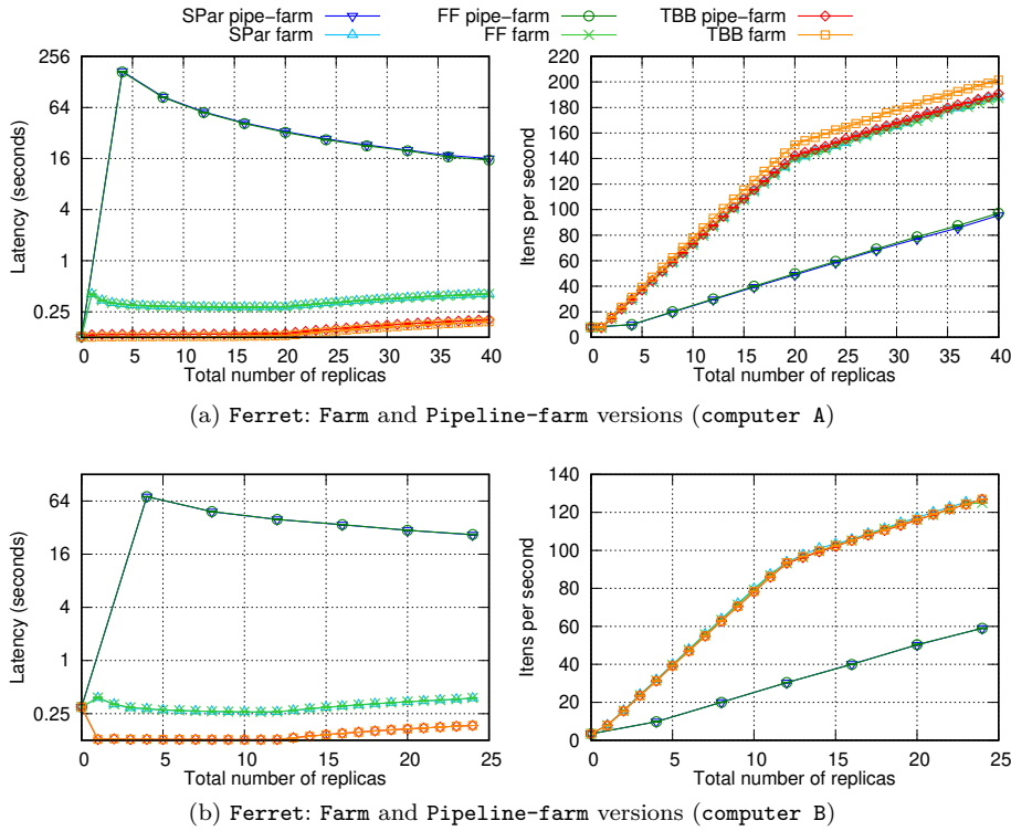
Fig. 6: Latency and throughput for the Farm and Pipeline of Farms compositions of Ferret. The pipe-farm versions have four Farms, so each increment of n increases four replicas at once.
