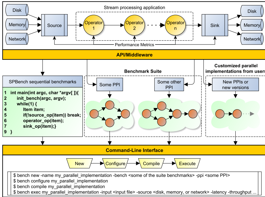
Fig. 2: SPBENCH framework.
