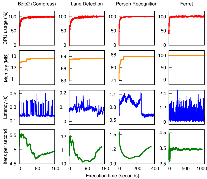
Fig. 4: Characterization results for the sequential applications.
