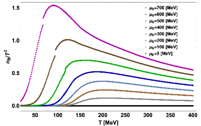
FIG. 7. Baryon density as a function of the temperature for different baryon chemical potentials. As expected, a discontinuity appears when \mu_B > \mu_{BC} , where the transition is first order. The critical point is located at \mu_{BC} = 500 MeV, resulting in T_C = 117 MeV and \alpha_1 = 11^\circ . Additionally, we have w = 15 , \rho = 0.3 , and \alpha_{12} = \alpha_1 , meaning \alpha_2 = \alpha_1 - \alpha_{12} = 0 .
