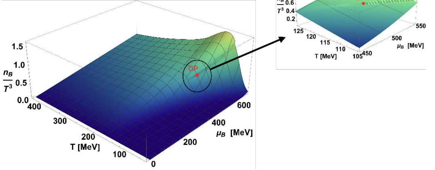
FIG. 13. Baryon density as a function of temperature and chemical potential for the same parameters as in Fig. 7, with a zoom into the critical region.
