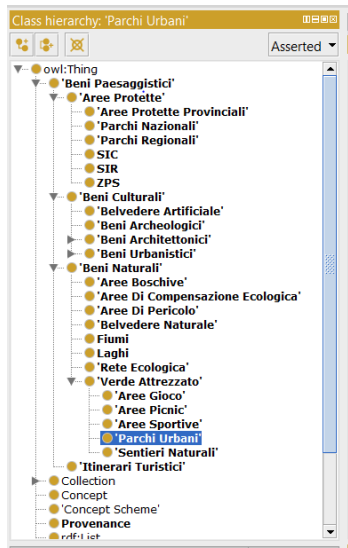
Figure 1: Portion of the OnToMap Ontology, visualized using the Protégé editor (stanford.protege.edu).
