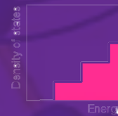
quantum well
