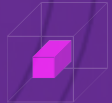
quantum dot
