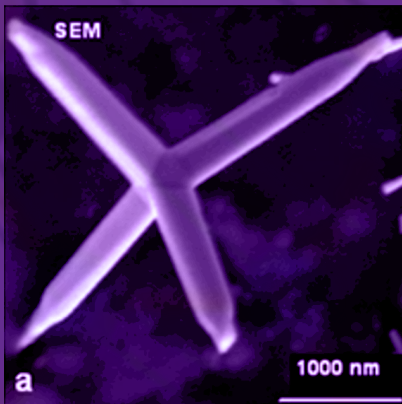
bulk
