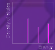
quantum dot
