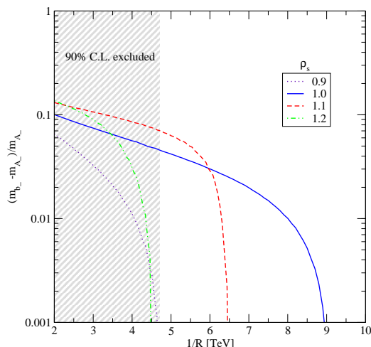
Figure 5: Correlation between the A_{-}^{(1)} – b_{-}^{(1)} mass splitting and compactification radius in models with \Omega h^2 matching the best fit value from cosmological observations for a few values of \rho_s .
