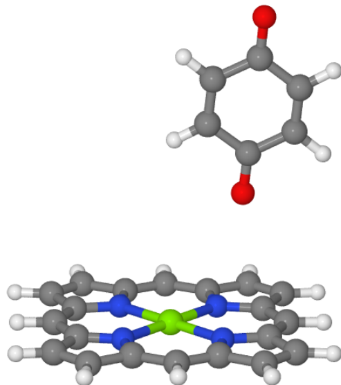
Figure 1. Structure of the Mg-porphyrin-benzoquinone donor-acceptor pair as used in the electronic-structure calculations. The complex has C_s symmetry.
