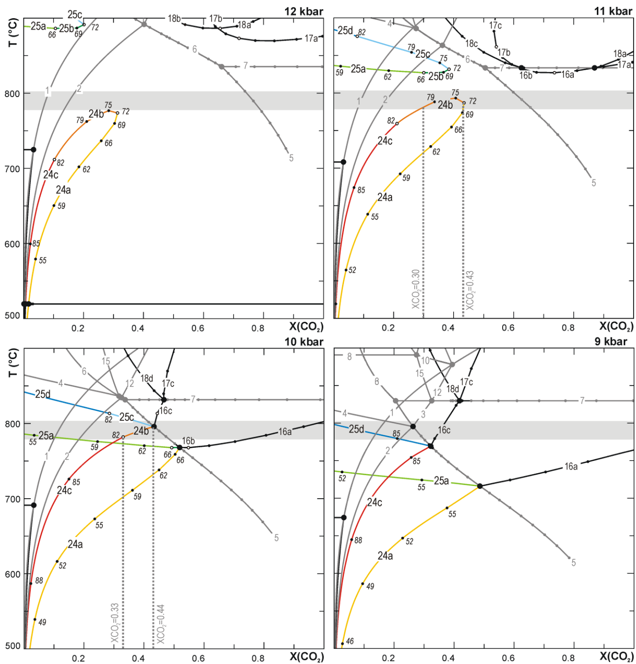
Fig. 12 – Isobaric T-X(CO 2 ) phase diagrams sections in the system CFAS-H 2 O-CO 2 at pressures from 12 to 9 kbar, calculated for a_{Hed} = 0.6 and a_{Me} = 0.8 . Thick line: univariant reactions; solid large point: invariant points; empty point: singular points and singular compositions (% Grs); solid small points indicate the variation of garnet composition along the univariant curves (% Grs, in italic). Equilibrium curves and points reported in grey refer to the degenerate reactions in the CAS-H 2 O-CO 2 system. Reaction labels as in Fig. 7. The shaded area corresponds to peak-T conditions as inferred from the hosting anatectitic paragneiss (see Groppo et al. 2009). The grey dotted lines constrain the composition of the fluid in equilibrium with garnet and quartz growing through reaction 24b (see text for discussion).
