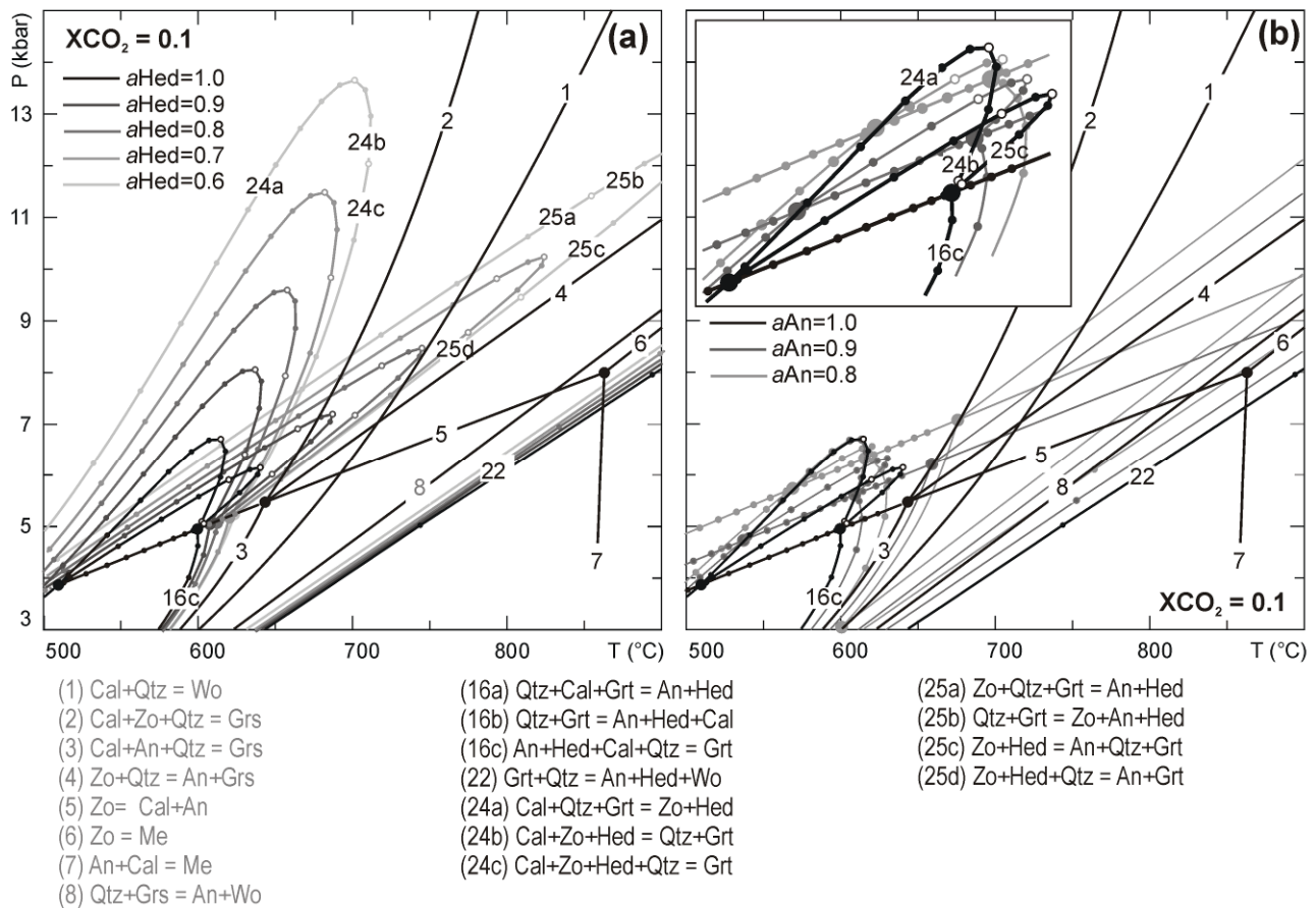
Fig. 8 – P-T phase diagrams in the system CFAS-H 2 O-CO 2 calculated at constant fluid composition of X(CO_2) = 0.1 and for different values of a_{Hed} (a) and a_{An} (b). The curves at a_{Hed}=1 and a_{An}=1 are the same as in the P-T phase diagram calculated at X(CO_2) = 0.1 in Fig. 7. Reaction labels as in Fig. 7. Equilibrium curves and points reported in grey refer to the degenerate reactions in the CAS-H 2 O-CO 2 system.
