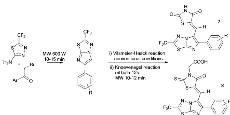
Scheme 5
