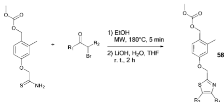
Scheme 39
