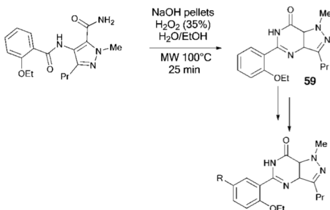
Scheme 40
