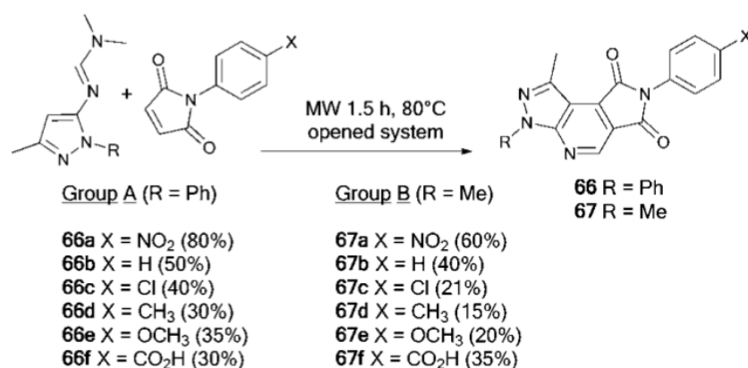
Scheme 46
