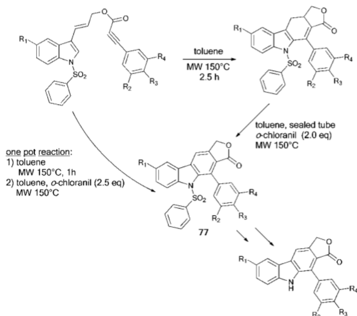
Scheme 53
