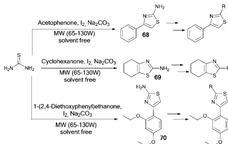
Scheme 47
