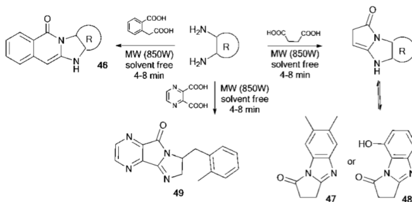
Scheme 34
