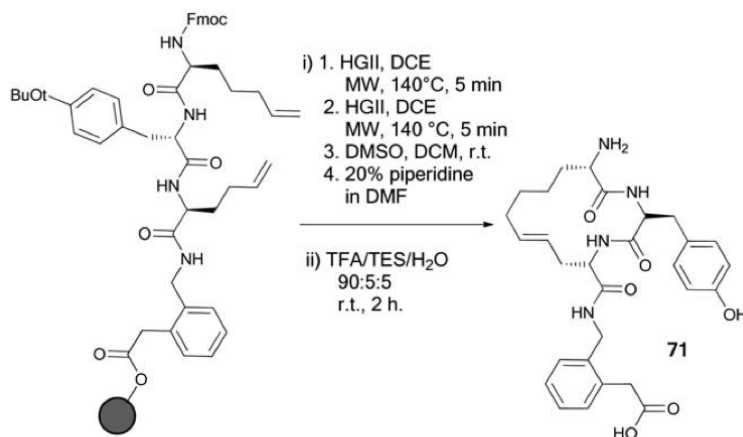
Scheme 48
