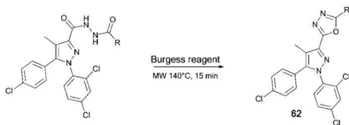
Scheme 43
