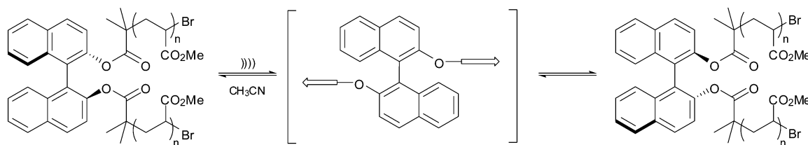
Scheme 10 Reconfiguration of chiral atropisomers by shear forces induced by sonication.
