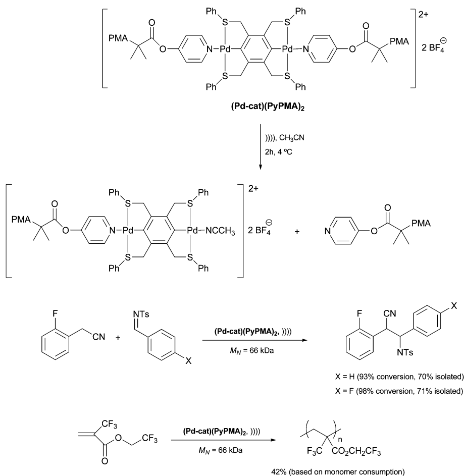
Scheme 15 Preparation of Pd–pyridine–PMA coordination polymers, which can be harnessed to promote, after sonication-induced cleavage, carbon–carbon bond-forming reactions and base-catalyzed polymerizations.
