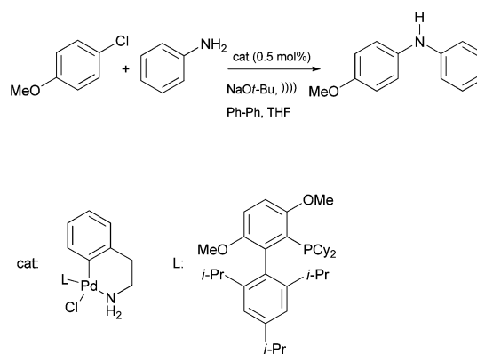
Scheme 4 Pd-catalyzed amination reactions to give diarylamines.
