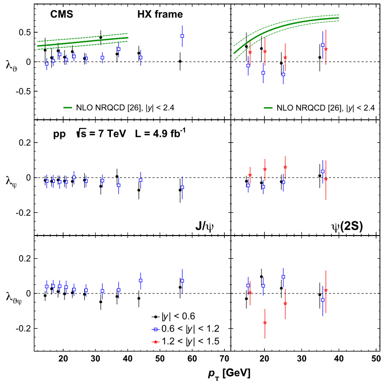
Fig. 6. Polarization parameters \lambda_{J/\psi} , \lambda_{\psi(2S)} , and \lambda_{J/\psi\psi(2S)} measured in the HX frame for prompt J/\psi (left) and \psi(2S) (right) mesons, as a function of p_T and for several |y| bins. The error bars represent total uncertainties (at 68.3% CL). The curves in the top two panels represent calculations of \lambda_{J/\psi} from NLO NRQCD [26], the dashed lines illustrating their uncertainties.
