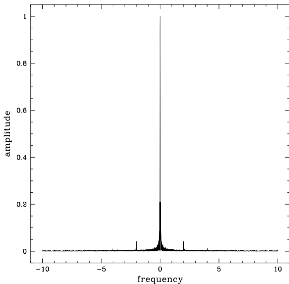
Fig. 5. Window function of CoRoT-33.
