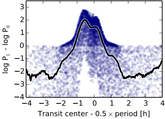
Fig. 11. Differences between the individual posterior samples for the eclipse model ( M_1 ) and no-eclipse model ( M_0 ) plotted against the eclipse centre (light blue circles), mapped from the sampling space that uses eccentricity and argument of periastron. Only 447 LC segments are used for the modelling (see Sect. 5.2). A Bayes factor map produced by sliding a uniform prior with a width of 15 minutes along the transit centre is overlaid with a black thick line.
