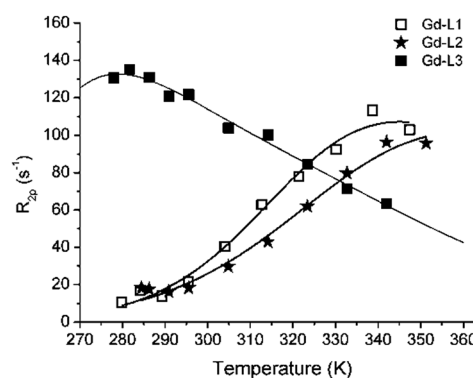
Fig. 2 Temperature dependence of the paramagnetic contribution to the ^{17}\text{O} transverse relaxation rate of water for Gd L1 , Gd L2 and Gd L3 (10 mM) measured at 2.1 T and pH 7.
