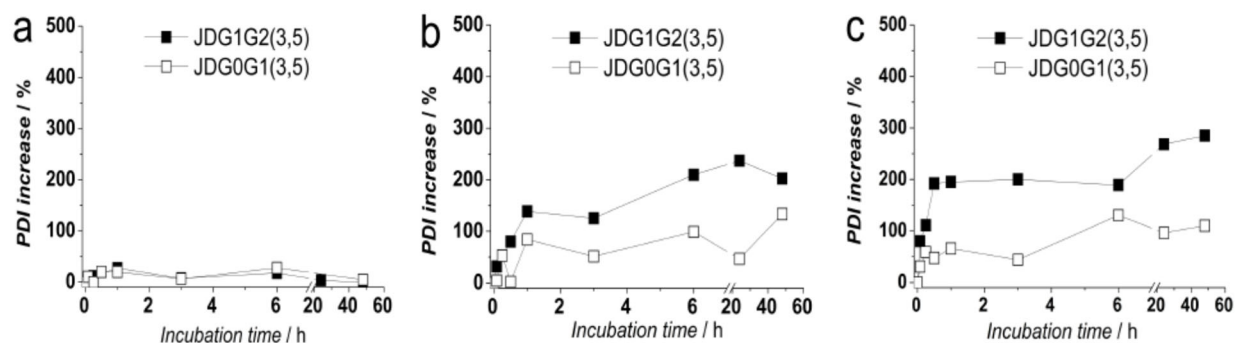
Figure 5. Changes in dimensional homogeneity. Percentage variation of the Polidispersity Index (PDI) of dendrimersomes as a function of incubation times at 37°C with a) isotonic buffer, b) Human Serum, and c) Human Serum Albumin.
