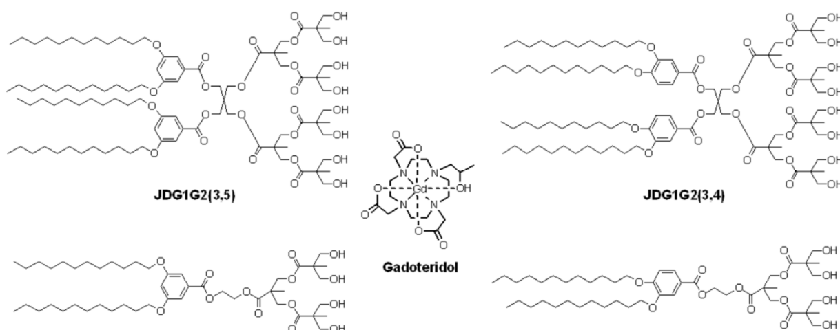
Figure 1. Chemical structures of Gadoteridol (in the center) and of the Janus dendrimers investigated in this work: JDG1G2(3,5) (top left), JDG1G2(3,4) (top right), JDG0G1(3,5) (bottom left), JDG0G1(3,4) (bottom right).
