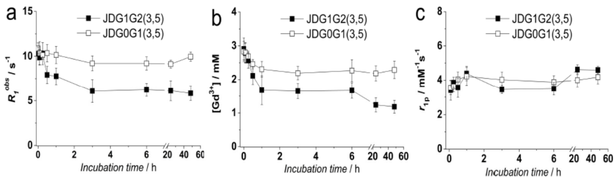
Figure 3. In vitro stability of (3,5)JD-based dendrimersomes in Human Serum. a) Water protons longitudinal relaxation rate ( R_{1obs} ) of different suspensions of dendrimersomes in human serum (HS) as a function of the incubation time at 37 °C. R_{1obs} was measured on the samples after dialysis. b) Residual concentration of Gd^{3+} in the sample, and c) normalized longitudinal relaxivity ( r_1 ) at each time point.
