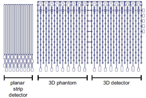
Figure 1: Mask for the metallisation of the diamond sample [4]. It is divided into three parts. On the right a strip structure to connect all conductive channels (“3D detector”), which is repeated in the middle but without conductive channels underneath (“3D phantom”) and on the left a planar strip detector.
