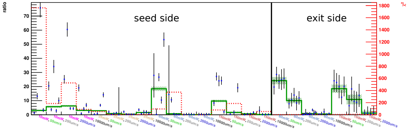
Figure 3: Ratio of the value of the diamond peak to the value of the g-peak. Results for individual channels are marked by a blue cross, the weighted mean for each setting is indicated by the green line. The red dotted line shows the \chi^2 value for each setting (for a coloured version of the plot the reader is referred to the web version of this paper).
