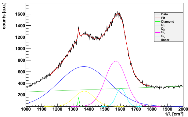
Figure 4: Raman spectrum for the seed side of a channel grown at 60 mW and 2,000 \mu\text{m s}^{-1} . Individual contributions of the fitted functions are shown.
