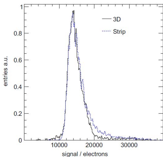
Figure 2: Charge spectra from the 3D detector and from the strip detector [4]. The peak of the distribution is for the 3D detector at 13,900 e and for the strip detector at 13,800 e. The mean values are 15,000 e and 15,800 e for the 3D and for the strip detector, respectively.
