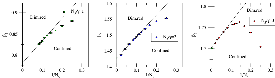
Figure 1. The effect of the discretization due to finite N_5 on the pseudo-critical coupling \beta_c(N_5/\gamma) . The phase transition breaks the center symmetry of the Polyakov loop along the extra dimension, such that \langle P_5 \rangle vanishes in the confining phase but has a non-zero expectation value in the dimensionally reduced phase. The pseudo-critical coupling is defined through the maximum of the susceptibility \chi_5 = \langle |P_5|^2 \rangle - \langle P_5 \rangle^2 .
