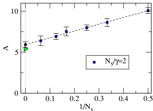
Figure 5. The coefficient A describing the exponential decay of the string tension as a function of the five-dimensional bare coupling, \sigma a^2 \sim \exp(-A\beta) , as a function of N_5 . The green triangle denotes the one-loop perturbative prediction as given by eq. (4.9). For lattices coarse in the fifth dimension, the coefficient differs by a factor of two, but approaching the continuum limit in the fifth dimension improves the agreement significantly.
