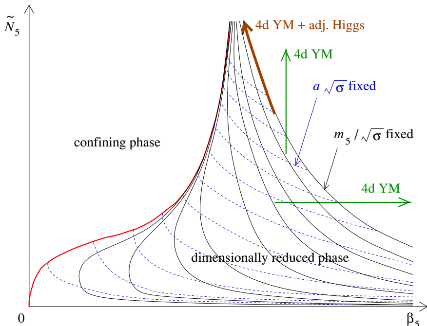
Figure 7. Sketch of the lines of constant low-energy physics (labelled by the m_5/\sqrt{\sigma} ratio) in the (\beta_5, \tilde{N}_5) phase diagram figure 2 of the 5d lattice model after taking the continuum limit in the fifth direction only. The red, leftmost, line indicates the phase transition separating the confining and the dimensionally reduced phases of the lattice theory. The lines of constant physics are displayed as solid black lines; at large \beta_5 values, they tend to hyperbolae of equation \beta_5 \tilde{N}_5 = \text{const} . The dashed blue lines correspond to fixed values of \sigma a^2 : the lattice spacing a decreases when \beta_5 \rightarrow \infty at fixed \tilde{N}_5 (green horizontal arrow), or when \tilde{N}_5 \rightarrow \infty at fixed \beta_5 (green vertical arrow). In both these limits the A_5 field decouples, and one recovers the ordinary continuum limit of the 4d YM theory. On the contrary, a continuum limit including 4d YM coupled to an adjoint scalar Higgs can be obtained by moving upwards along a line of fixed m_5/\sqrt{\sigma} (brown arrow). Finally, observe that, for any fixed, finite value of \sigma a^2 (i.e. on any dashed blue line), there is a finite maximum value of \tilde{N}_5 , i.e. a finite maximum value of L_5/a , which is reached at the \beta_5 value where the dashed blue line hits the phase transition line.
