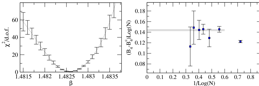
Figure 9. On the left-hand panel, the reduced \chi^2 -value of the fitting ansatz eq. (A.5), applied to the data of figure 8 (the points corresponding to N = 4 were not included in the fit). On the right-hand panel, the data at \beta = 1.4826 are well described by the ansatz eq. (A.5), with \chi^2/\text{d.o.f} = 0.50(7) and quickly deteriorates away from this point, which we take as our estimate of the critical point.
