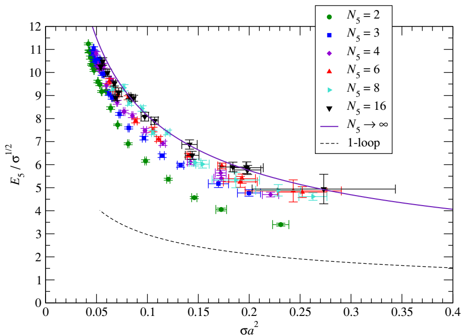
Figure 6. Simulation results for the Higgs screening mass E_5 extracted from the exponential decay of the zero-momentum correlator of the Polyakov loop in the fifth direction, eq. (4.11), versus the string tension in units of the lattice spacing. The screening mass E_5 is expressed in units of the square root of the 4d string tension, and is given by E_5 = 2m_5 to leading order in perturbation theory. The figure shows our data at fixed \tilde{N}_5 = N_5/\gamma = 2 and for different N_5 values. The solid curve is obtained by extrapolation to the N_5 \rightarrow \infty limit. While the data show qualitative agreement with the one-loop perturbative prediction (thin dashed line), the quantitative details differ due to moderate values of the bare coupling \beta .
