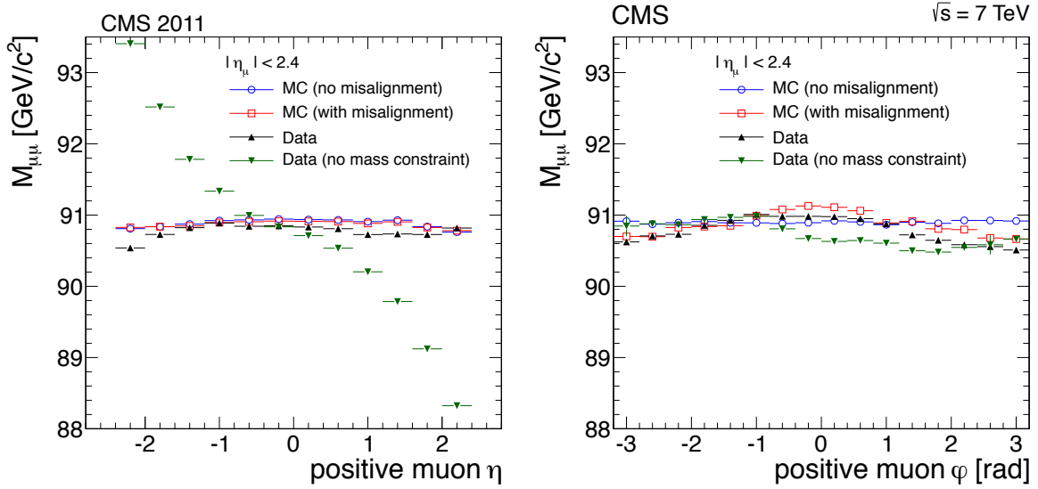
Figure 16: Invariant mass of Z \rightarrow \mu^+ \mu^- candidates as a function of \eta (left) and \varphi (right) of the positively charged muon. Distributions from aligned data are shown as black upward-pointing triangles. Distributions from a simulation without misalignment and with realistic misalignment (see section 5) are presented as blue hollow circles and red hollow markers, respectively. The same distribution with the data but with a geometry produced without using the Z-boson mass information is presented with green downward-pointing triangles.
