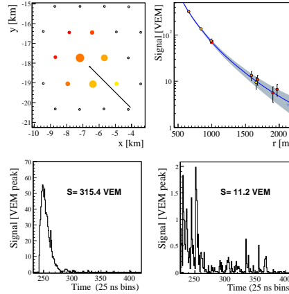
Figure 17: Event 13357690: a typical vertical event of about 3 \times 10^{19} eV. Top left : The array seen from above with the 8 triggered stations. Top right : The fit to the lateral distribution function (LDF) for this shower of zenith angle 28^\circ . Bottom : The FADC traces from 2 detectors at distances of 650 and 1780 meters from the shower core. The signal sizes are in units of VEM.
