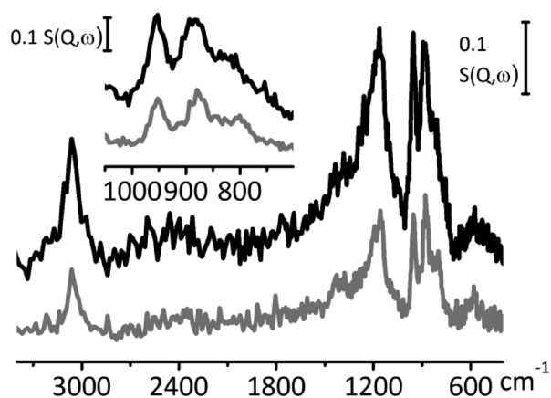
Fig. 7 Incoming proton current and mass normalised INS spectra of C_W (grey) and C_{\text{Chem}}i (black) carbons ( S(Q, \omega) as a function of the energy transfer in \text{cm}^{-1} ). The inset shows a magnification of the 1050\text{--}600\text{ cm}^{-1} range.
