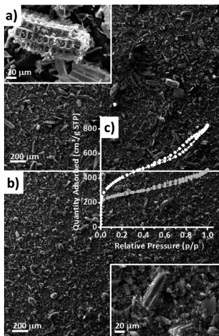
Fig. 1 Representative SEM images of C_W (a) and C_{\text{Chemical}} (b). (c) N_2 physisorption isotherms collected at 77 K for C_W (grey) and C_{\text{Chemical}} (white).
