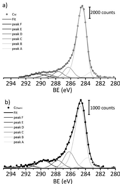
Fig. 5 High-resolution XPS spectra of C 1s peak for C_W (part a) and C_{\text{Chemical}} (part b) and corresponding fits with six Gaussian components. For details see Tables S2 and S3.†
