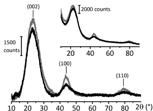
Fig. 2 XRPD patterns of C_W (grey) and C_{\text{Chemical}} (black) carbons after subtraction of the background and assignment of the main peaks ( \lambda = 1.5409 \text{ \AA} ). The inset shows the patterns as collected.
