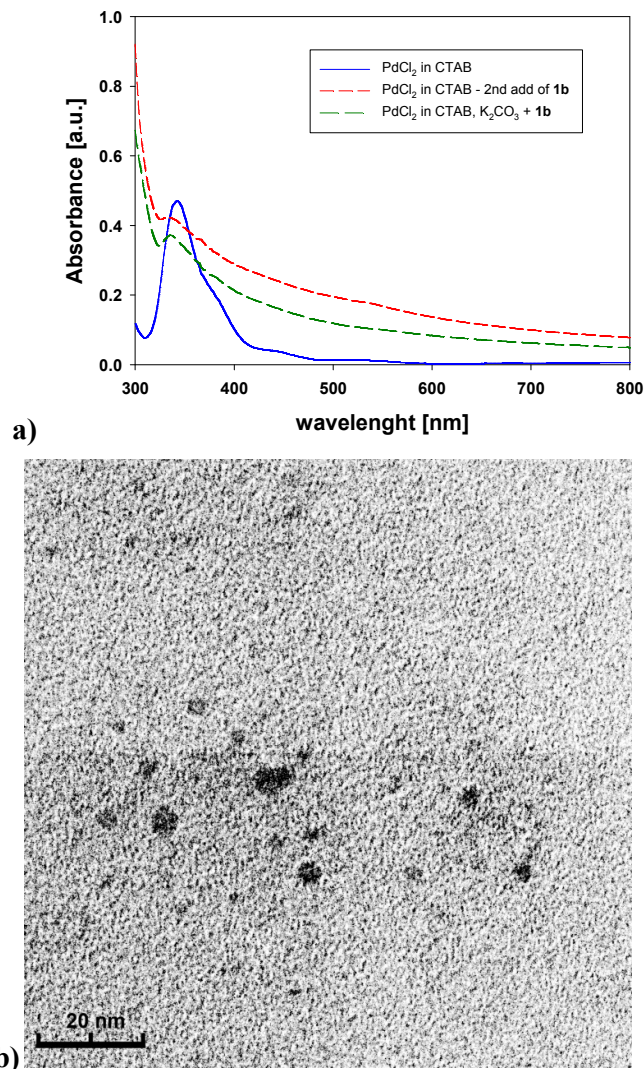
Figure 6. Panel a: UV spectra for PdCl 2 in CTAB (blue, solid line); in CTAB after the second addition of 1b (red, short dash line); in CTAB and K 2 CO 3 after a first addition of 1b (green, medium dash line). Panel b: TEM image of the Pd nanoparticles formed by Pd reduction in the solution showing UV spectrum marked in red in Panel a.
