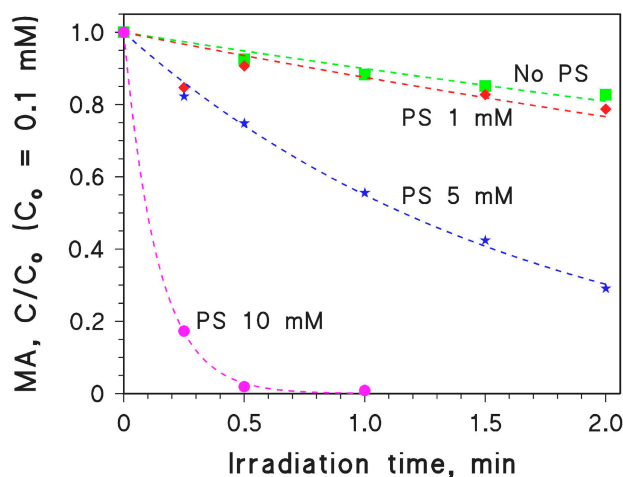
Figure 3. Time trend of 0.1 mM MA upon UVC irradiation, alone or in the presence of different concentration values of Na 2 S 2 O 8 (persulphate, PS). The PS concentration was varied in the range of 0–10 mM.
