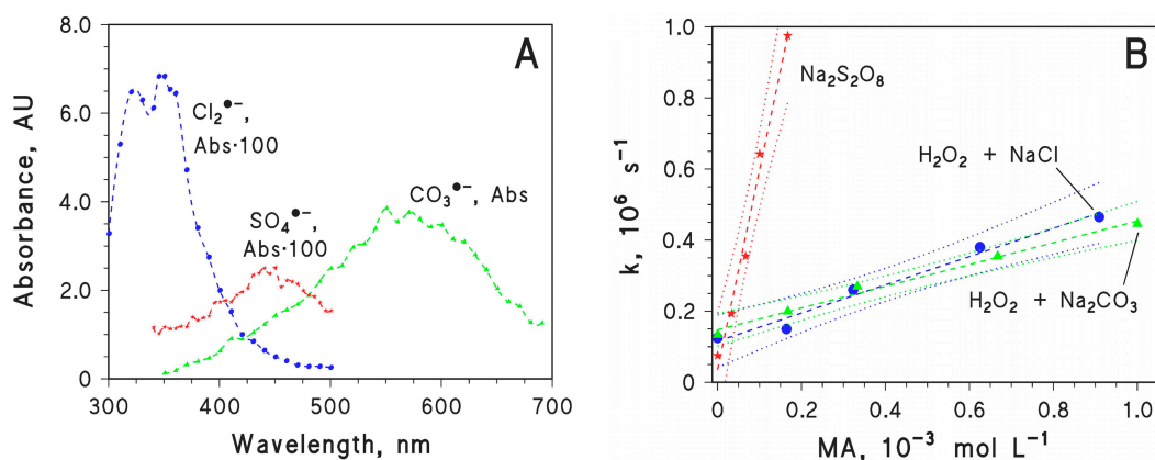
Figure 4. (A) Absorption spectra of the radicals \text{CO}_3\cdot^- , \text{Cl}_2\cdot^- , and \text{SO}_4\cdot^- produced by laser flash photolysis of 2.5 mM \text{H}_2\text{O}_2 + 0.1 M \text{Na}_2\text{CO}_3 ( \text{CO}_3\cdot^- ), of 2.5 mM \text{H}_2\text{O}_2 + 0.01 M \text{NaCl} (pH 3, adjusted with \text{HClO}_4 ) ( \text{Cl}_2\cdot^- ), and of 10 mM \text{Na}_2\text{S}_2\text{O}_8 ( \text{SO}_4\cdot^- ). The absorbance signals were taken soon after the laser pulse. Laser irradiation at 266 nm, 35 \text{ mJ}\cdot\text{pulse}^{-1} ; (B) First-order decay constants of the studied radical species ( \text{SO}_4\cdot^- , \text{Cl}_2\cdot^- , \text{CO}_3\cdot^- ) as a function of MA concentration. The radical species were obtained by laser irradiation of 10 mM \text{Na}_2\text{S}_2\text{O}_8 ( \text{SO}_4\cdot^- ), of 2.5 mM \text{H}_2\text{O}_2 + 0.01 M \text{NaCl} at pH 3 ( \text{Cl}_2\cdot^- ), and of 2.5 mM \text{H}_2\text{O}_2 + 0.1 M \text{Na}_2\text{CO}_3 ( \text{CO}_3\cdot^- ). The slopes of the lines give the second-order reaction rate constants between the relevant radicals and MA (Stern-Volmer approach).
