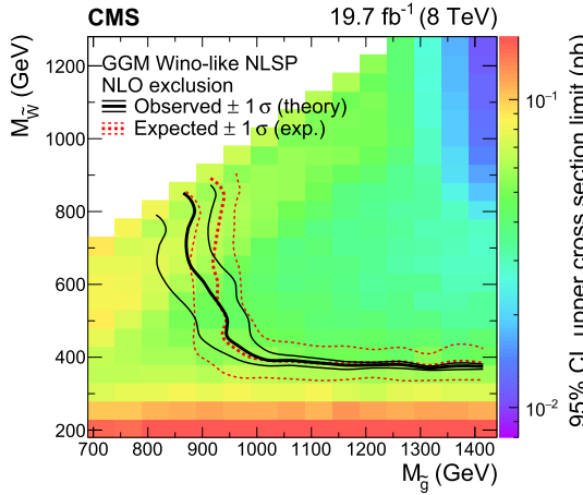
Fig. 5. Observed and expected 95% confidence level upper limits on the cross section and corresponding exclusion limits for the GMSB model.
