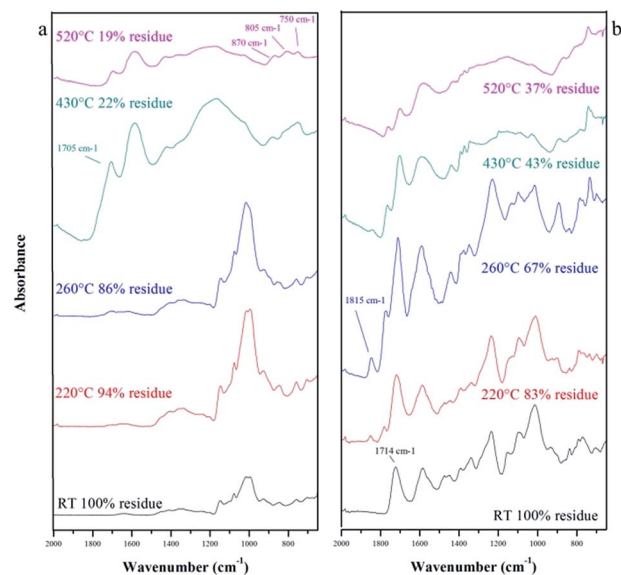
Fig. 6 ATR spectra collected at different temperatures for the LC (a) and LNS (b).
