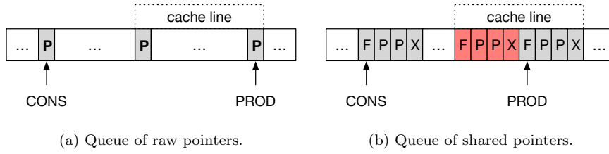
Fig. 4: Synchronization flags are denoted by F, whereas P represents a shared pointer word and X are padding words.
