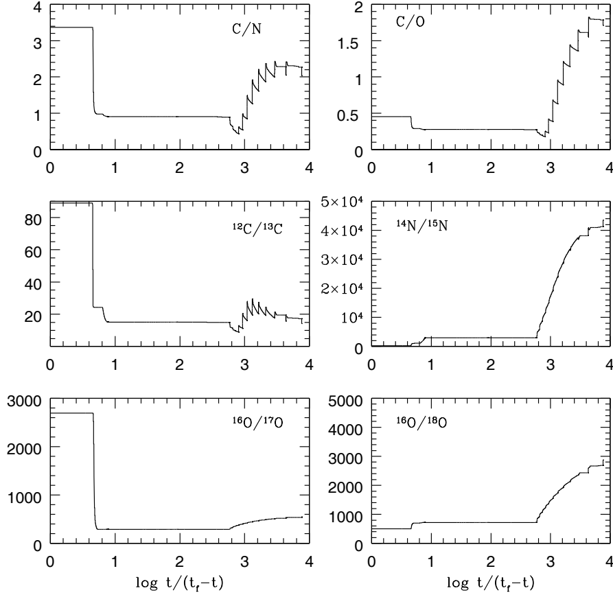
Fig. 7. Evolution up to the AGB tip of C, N, and O elemental and isotopic ratios in a 2 M_{\odot} model with both RGB and AGB extra mixing. In the first case the maximum temperature was fixed to T_{\max} = 22 MK, while in the latter T_{\max} = 40 MK (see text for further details). The evolutionary timescale was rescaled to t_f = 1.196 Gyr, which corresponds to the age of the last computed model (AGB tip). The FDU occurs at \log t/(t - t_f) \sim 0.7 , while some effect of the RGB extra mixing is visible a bit later. Finally the combined actions of the and the AGB extra mixing arise at \log t/(t - t_f) > 2.8 .
