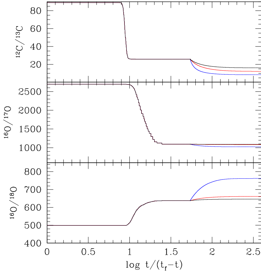
Fig. 6. Evolution up to the RGB tip of C and O isotopic ratios in the 3 models with extra mixing described in the text. The maximum temperature attained by extra mixing is T_{\max} = 20, 21 , and 23 MK (black, red, and blue lines, respectively). In all cases, the fluid velocity in the extra-mixing zone is about 1/100 of that in the fully convective envelope. The evolutionary timescale has been properly rescaled to t_f = 2.91 Gyr, which corresponds to the onset of the core-He burning. The FDU starts at \log t/(t - t_f) \sim 1 , while the extra-mixing process is activated just after \log t/(t - t_f) \sim 1.7 , namely, the epoch of the RGB bump.
