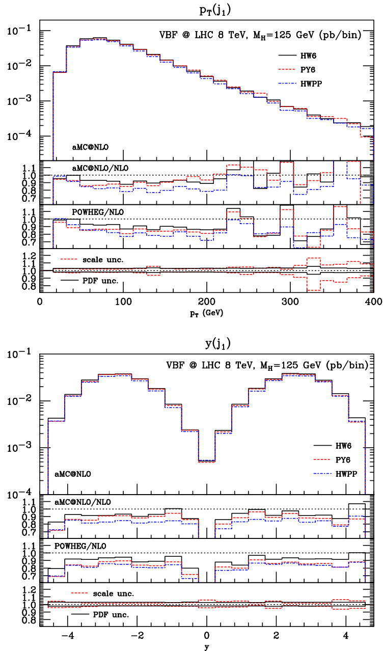
Fig. 2. Same pattern as in Fig. 1; for the hardest-jet transverse momentum (top) and rapidity (bottom).
