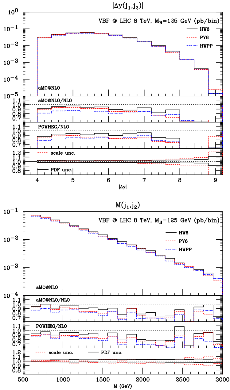
Fig. 5. Same pattern as in Fig. 1; for the rapidity separation (top) and invariant mass (bottom) of the two hardest jets.
