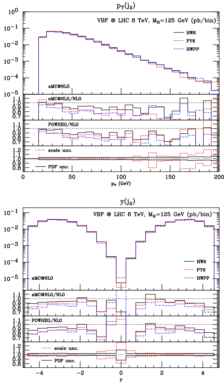
Fig. 3. Same pattern as in Fig. 1; for the second hardest-jet transverse momentum (top) and rapidity (bottom).
