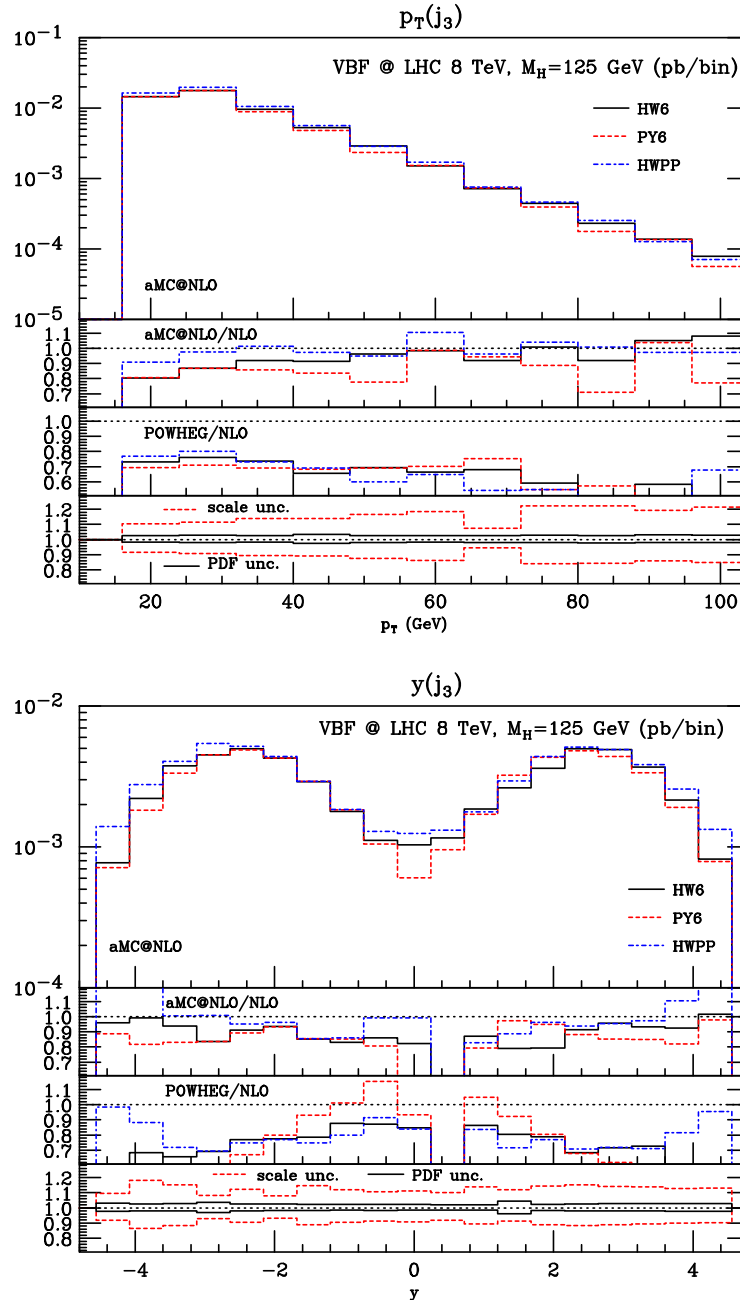
Fig. 6. Same pattern as in Fig. 1; for the third hardest-jet transverse momentum (bottom) and rapidity (top).
