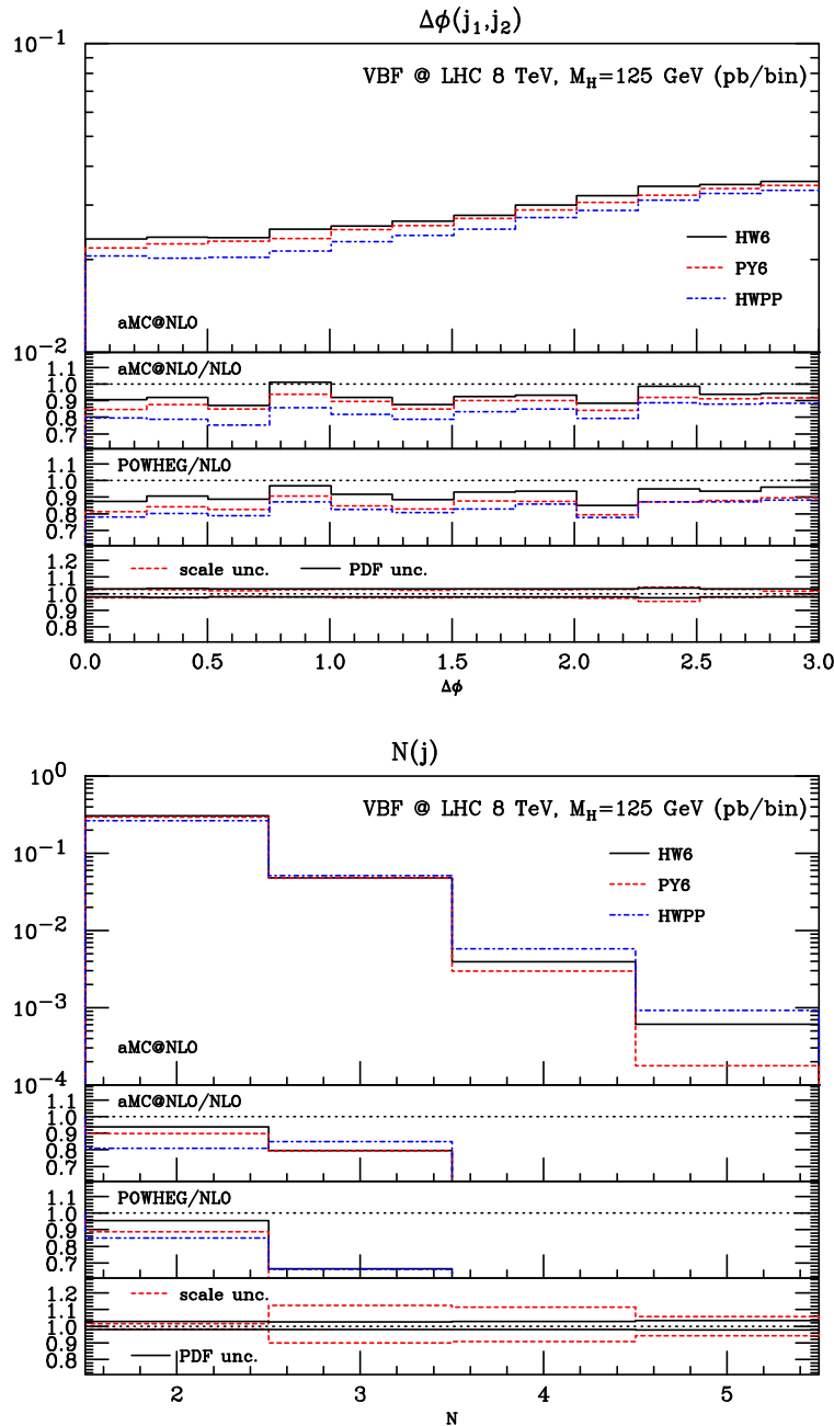
Fig. 4. Same pattern as in Fig. 1; for the azimuthal separation of the two hardest jets (top) and the exclusive jet-multiplicities (bottom).
