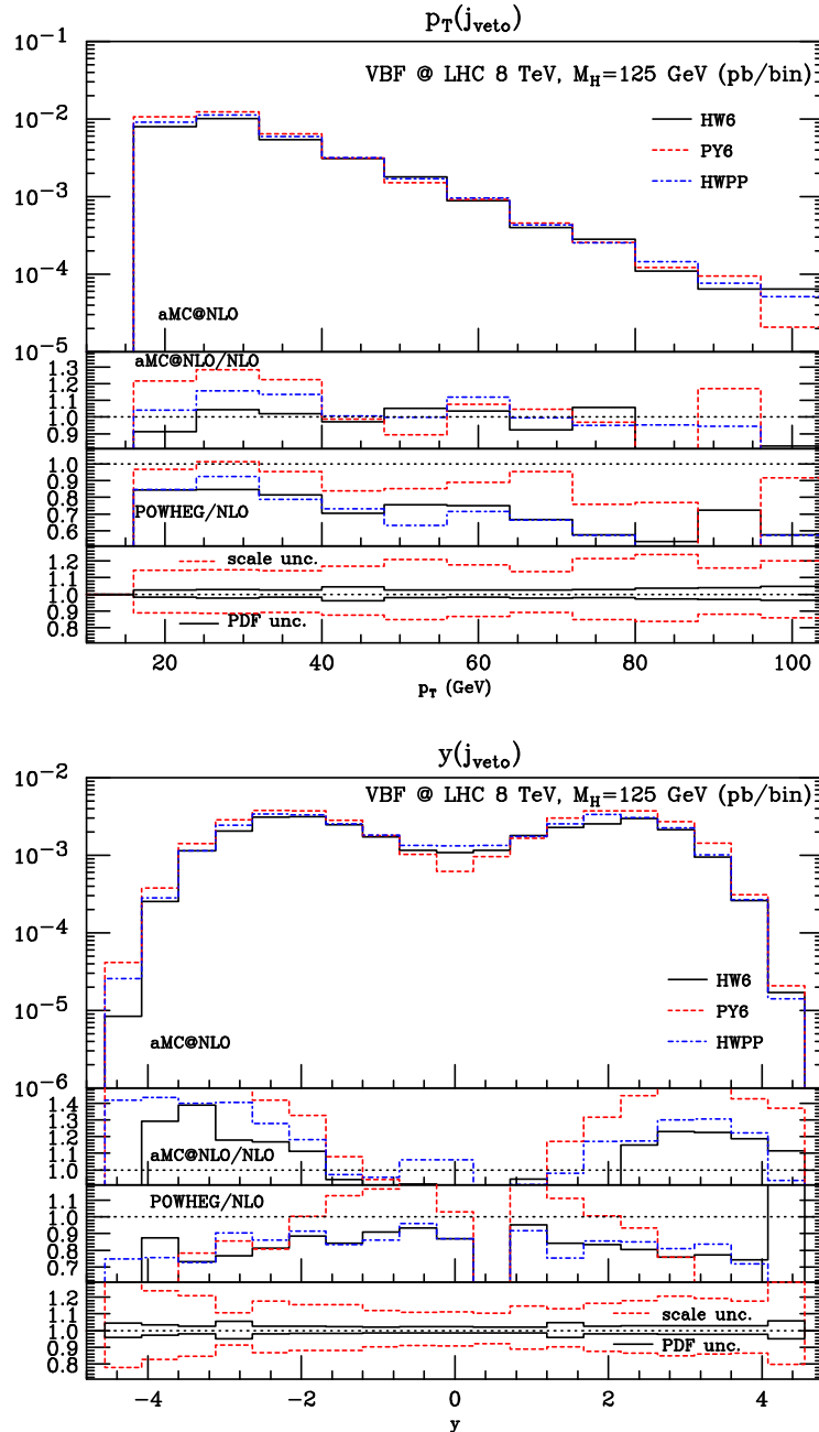
Fig. 7. Same pattern as in Fig. 1; for the veto-jet transverse momentum (top) and rapidity (bottom).
