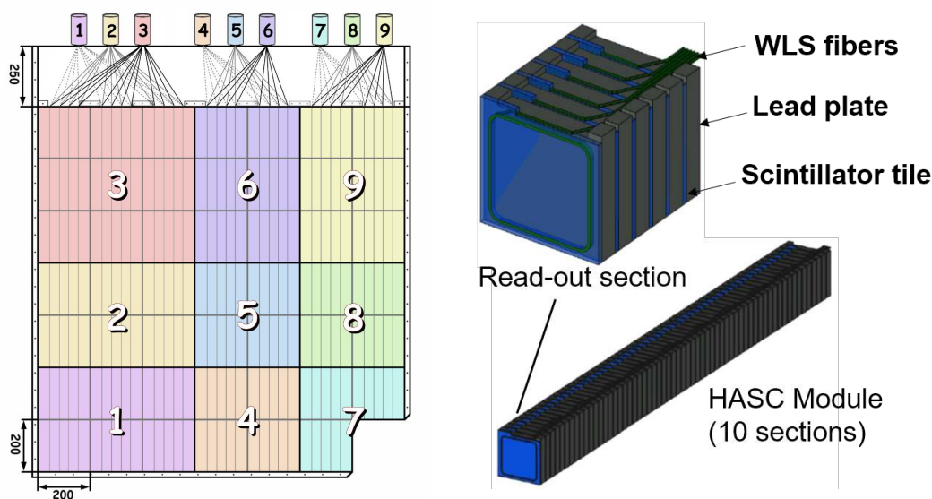
Figure 57. Left: sketch of the MUV0 detector showing the pattern of scintillator tiles and super-tiles. Right: a HASC module with 100 \times 100 \text{ mm}^2 cross section; six consecutive scintillators are connected to one optical fibre, leading to 10 fibres per module. Each fibre is read out with a SiPM.
