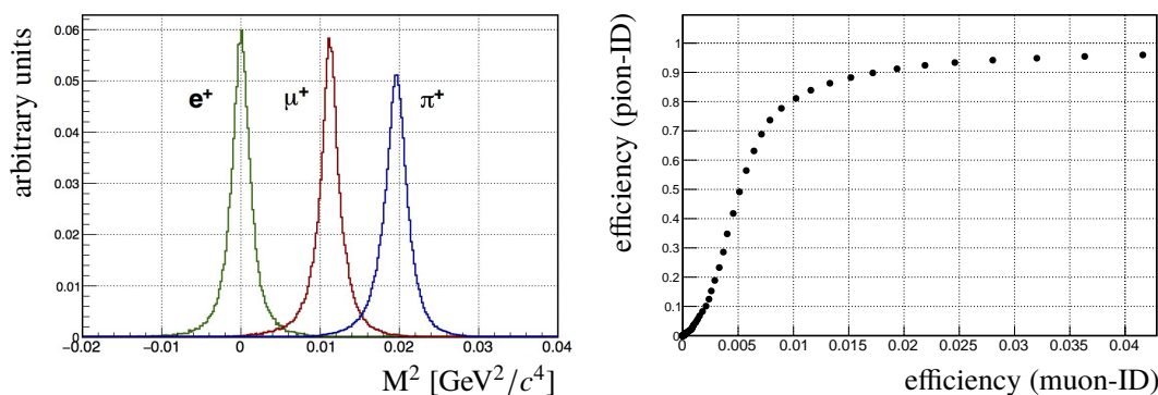
Figure 76. RICH particle identification for track momenta between 15 and 35 \text{GeV}/c . Left: squared particle mass reconstructed using the velocity estimated by the Cherenkov angle measured by the RICH and the momentum measured by the spectrometer, for positrons, muons, and charged pions selected using spectrometer and calorimetric information. Right: pion-ID efficiency versus muon-ID efficiency for different choices of the reconstructed mass range.
