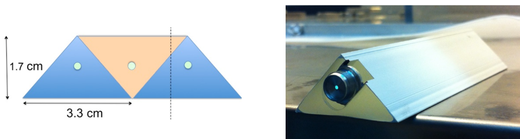
Figure 19. Left: arrangement of the bars to form a plane. Right: a triangular bar, constituting the building block of the CHANTI detector. The WLS fibre is visible in the centre.
