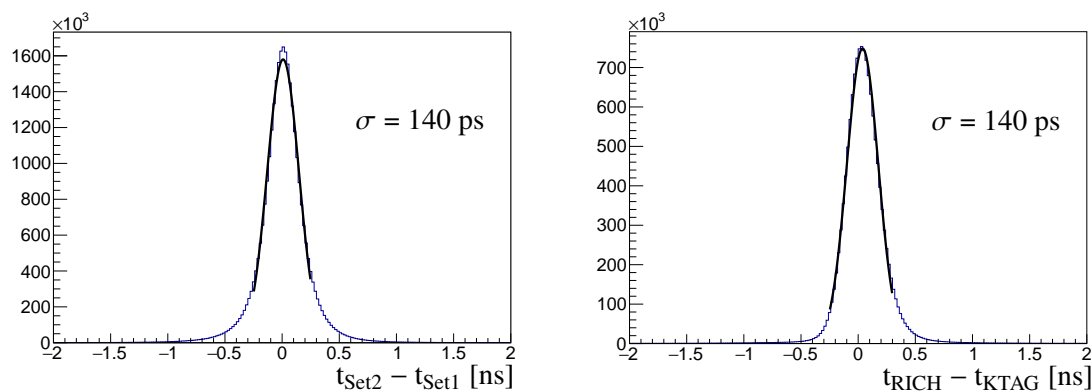
Figure 44. Left: intrinsic time resolution of the Cherenkov photons. The detected photons of one Cherenkov ring are divided into two groups and the time difference is plotted. The width of the Gaussian fit is 140 ps. The time resolution of the full ring is one half of this width. Right: time difference between the average time of a Cherenkov ring and the KTAG time. The width of the Gaussian fit is 140 ps.
