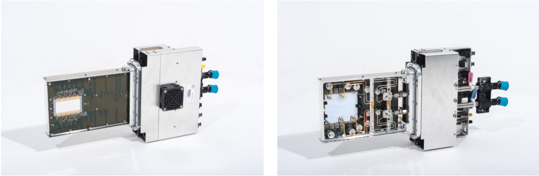
Figure 13. Picture of an assembled station looking at the sensor side (left) and at the cooling side (right).
