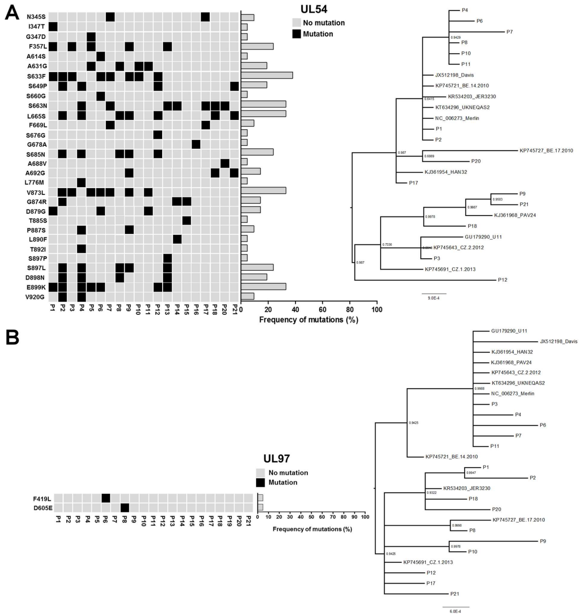
248 249 Fig. 5. Antiviral susceptibility testing. The heterogeneity of UL54 (A) and UL97 (B) genes is reported. 250 Left panel. The heat maps show the presence and the positions of amino acidic changes, and the 251 histograms show the frequency of each modification. Right panel. The Bayesian tree describes the 252 genetic relationship among samples based on nucleotide alignment.
