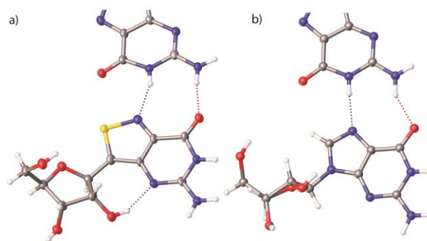
Figure 3. Comparison of intermolecular H-bonding seen in the crystal structures of (a) tG and (b) G .
