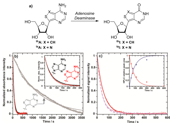
Figure 5. (a) Deamination of th A and u A (b) Enzymatic deamination of A to I (black), u A to u I (red) and th A to th I (grey) with ADA monitored by real-time absorption at 260, 340 and 340 nm respectively. Inset: zoomed in region between 0 and 300 seconds. (c) Enzymatic deamination of u A to u I by ADA monitored by real-time absorption (red) at 340 nm and real time emission (light purple) at 410 nm (excitation at 322 nm). Inset: HPLC relative peak area variation at different time-points for u A (red) and u I (blue) monitored at 340 nm
