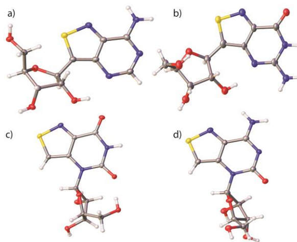
Figure 2. X-ray crystal structures of isothiazolo[4,3- d ]pyrimidine analogs: (a) tA (b) tG (c) tU (d) tC .
