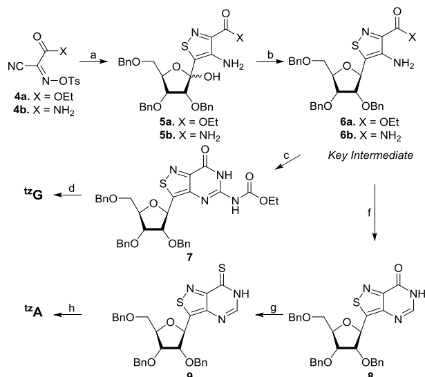
Figure 2. X-ray crystal structures of isothiazolo[4,3- d ]pyrimidine analogs: (a) tA (b) tG (c) tU (d) tC .
