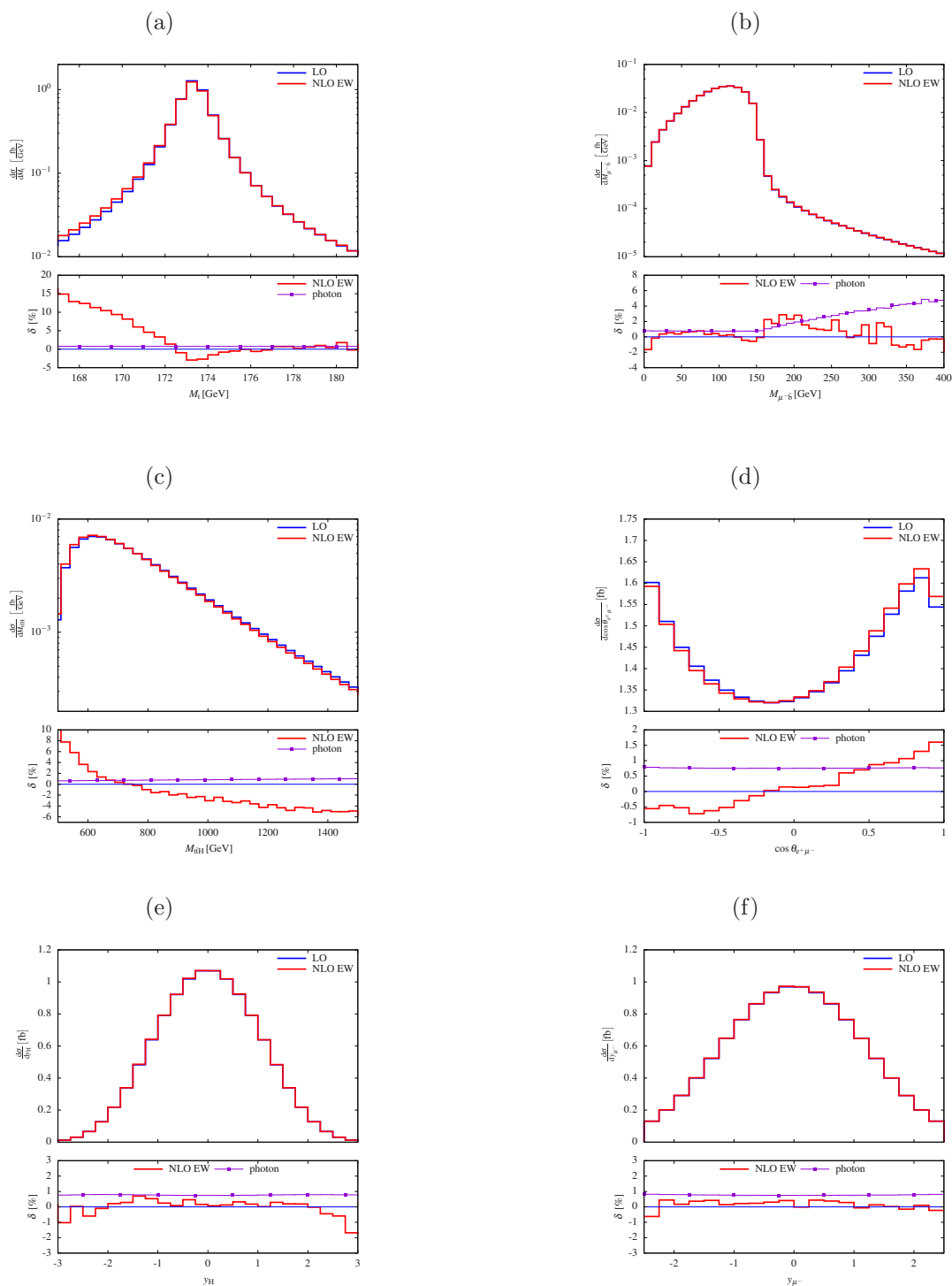
Figure 7. Distributions at the LHC running at a centre-of-mass energy \sqrt{s} = 13 TeV: (a) invariant mass of the reconstructed top quark (upper left), (b) invariant mass of the \mu^- \bar{\mu} system (upper right), (c) invariant mass of the reconstructed t\bar{t}H system (middle left), (d) cosine of the angle between the positron and the muon (middle right), (e) rapidity of the Higgs boson (lower left), and (f) rapidity of the muon (lower right). In the lower panels, the relative NLO EW corrections \delta = \sigma_{\text{NLO EW}}/\sigma_{\text{LO}} - 1 and the relative photon-induced contributions \delta = \sigma_{\gamma g}/\sigma_{\text{LO}} in per cent are shown.
