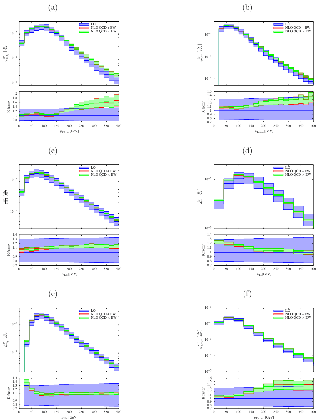
Figure 9. Combined NLO EW and QCD corrections for various distributions at the LHC running at a centre-of-mass energy \sqrt{s} = 13 TeV: (a) transverse momentum for the bottom-jet pair (upper left), (b) for the missing momentum (upper right), (c) for the Higgs boson (middle left) (d) for the reconstructed top quark (middle right) (e) for the harder bottom jet (lower left), and (f) for the e^+\mu^- system (lower right). In the upper panels the LO, the NLO QCD+EW and NLO QCD \times EW distributions are shown. The lower panels display the two differently combined NLO predictions with respect to the LO one as K = \sigma_{\text{NLO}}/\sigma_{\text{LO}} .
