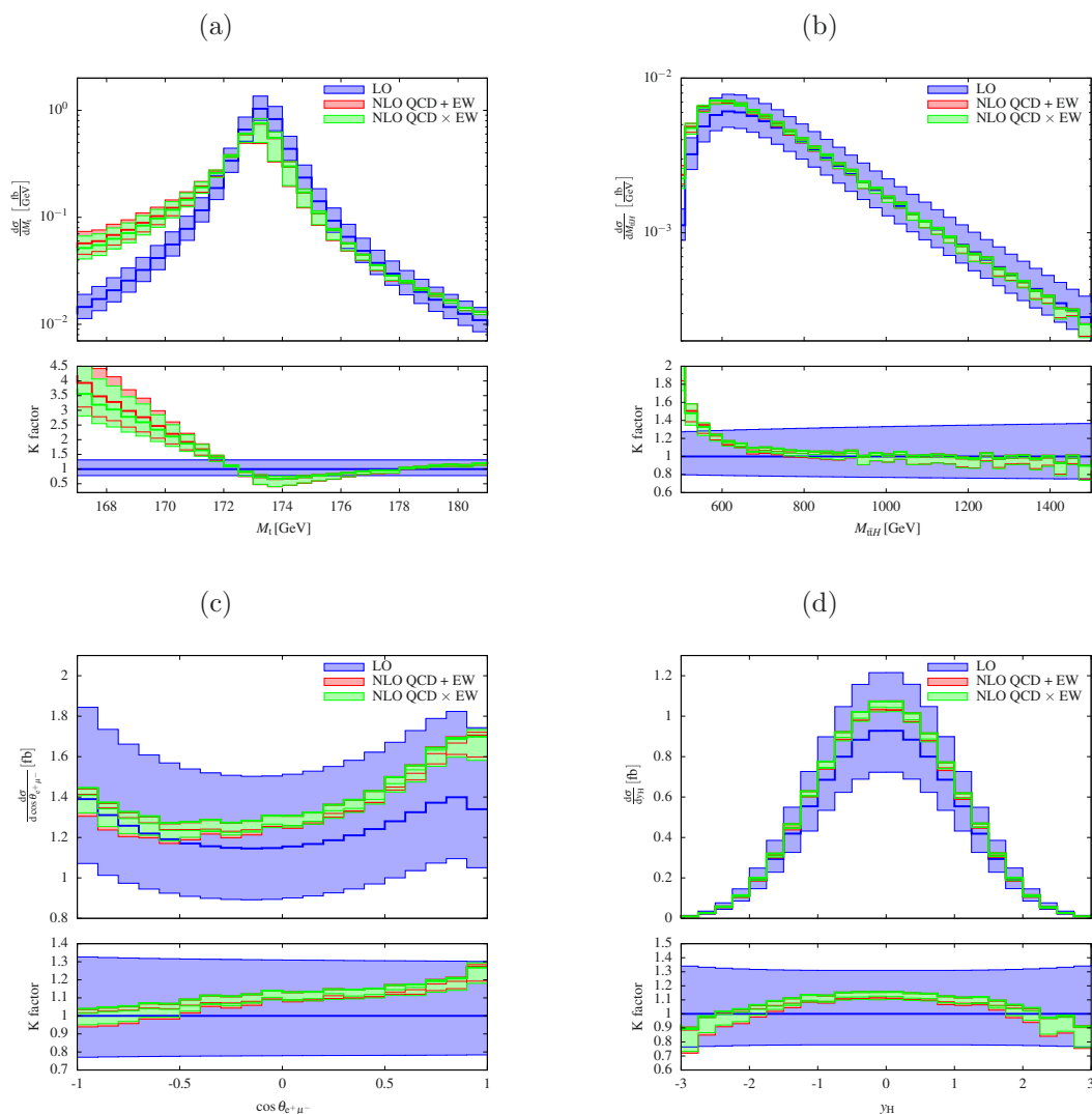
Figure 10. Combined NLO EW and QCD corrections for various distributions at the LHC running at a centre-of-mass energy \sqrt{s} = 13 TeV: (a) invariant mass of the reconstructed top quark (upper left), (b) invariant mass of the reconstructed t\bar{t}H system (upper right), (c) cosine of the angle between the positron and the muon (lower left) (d) rapidity of Higgs boson (lower right). In the upper panels the LO, the NLO QCD+EW and NLO QCD \times EW distributions are shown. The lower panels display the two combined NLO predictions with respect to the LO one as K = \sigma_{\text{NLO}}/\sigma_{\text{LO}} .
