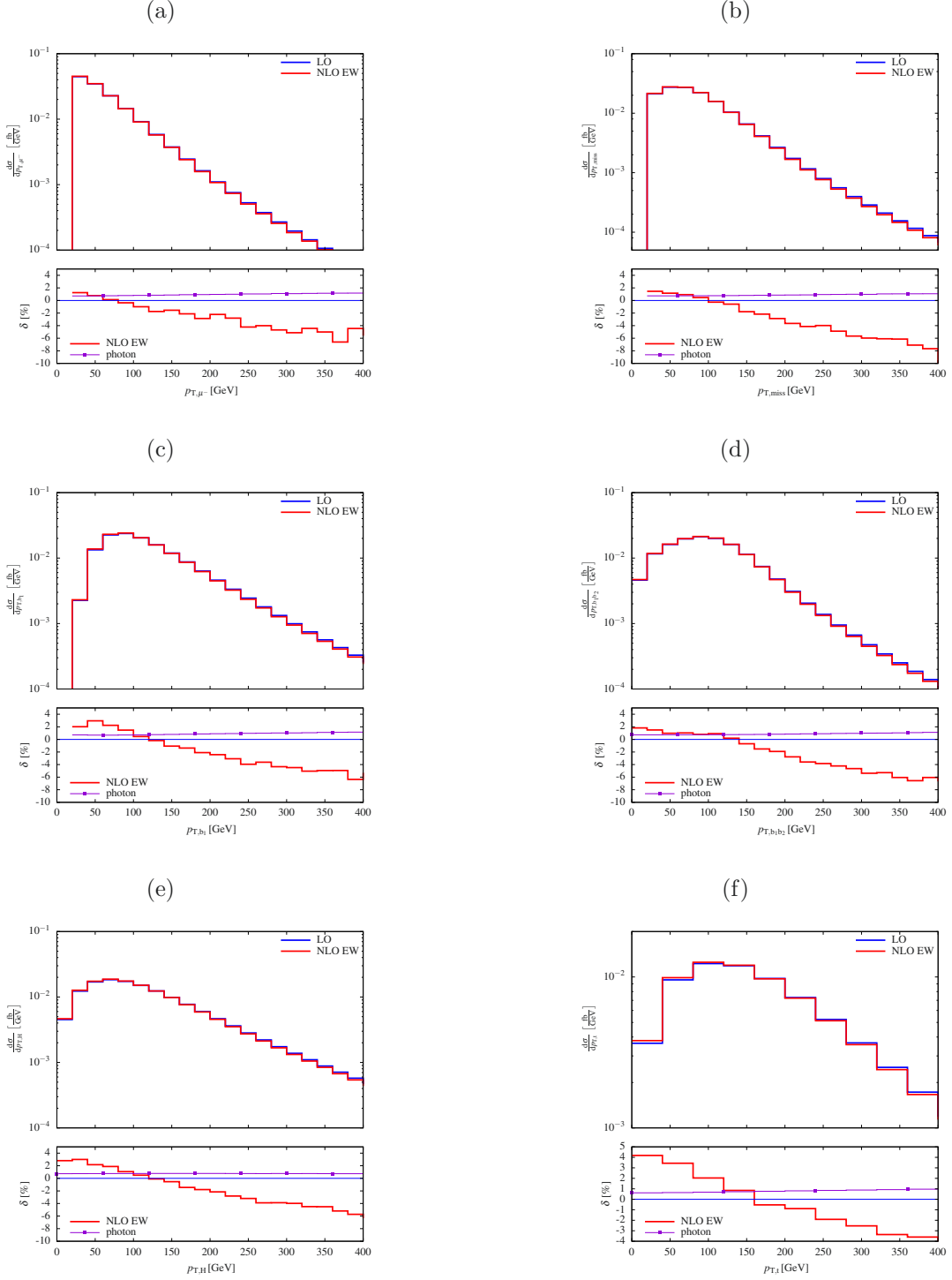
Figure 6. Transverse-momentum distributions at the LHC running at a centre-of-mass energy \sqrt{s} = 13 TeV: (a) for the muon (upper left), (b) for the missing momentum (upper right), (c) for the harder bottom jet (middle left), (d) for the bottom-jet pair (middle right), (e) for the Higgs boson (lower left), and (f) for the reconstructed top quark (lower right). In the lower panels, the relative NLO EW corrections \delta = \sigma_{\text{NLO EW}}/\sigma_{\text{LO}} - 1 and the relative photon-induced contributions \delta = \sigma_{\gamma g}/\sigma_{\text{LO}} in per cent are shown.
