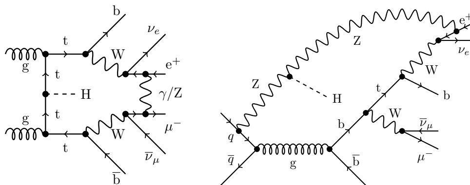
Figure 4. Sample one-loop Feynman diagrams squared. On the left-hand side, the diagram represents an EW correction to the QCD process which can also be seen as a QCD correction to the EW amplitude interfered with the QCD amplitude. On the right-hand side, a QCD correction to the QCD amplitude interfered with the EW amplitude is displayed. The decay products of the top quarks are not shown as their inclusion does not alter the discussion.
