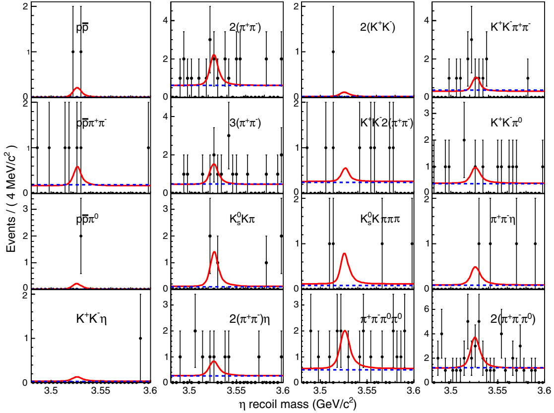
FIG. 2. Simultaneously fitted \eta recoil mass spectra in e^+e^- \rightarrow \eta h_c, h_c \rightarrow \eta \eta_c, \eta_c \rightarrow X_i for the 16 final states X_i at \sqrt{s} = 4.226 GeV. The dots with error bars represent the \eta recoil mass spectrum in data. The solid lines show the total fit function and the dashed lines are the background component of the fit.
