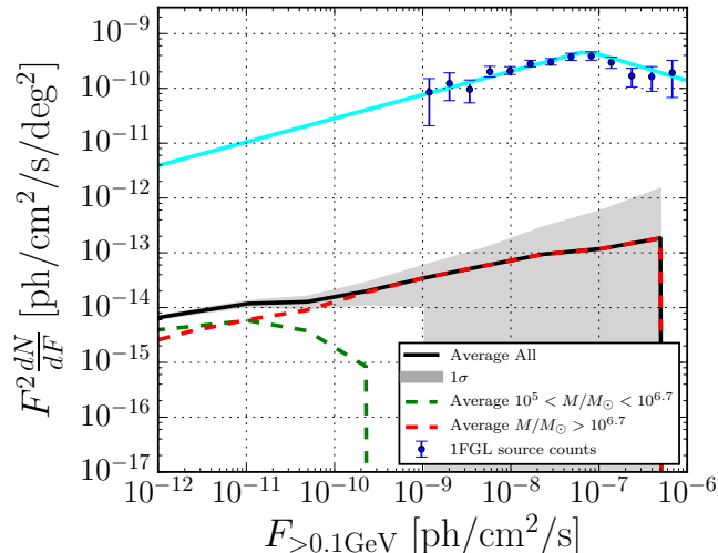
Figure 13. Same as left panel in figure 12, for M_{\text{SH}} \geq 10^5 M_{\odot} (mass resolution of AQ08). We show separately the contribution of 10^5 M_{\odot} \leq M_{\text{SH}} < 10^{6.7} M_{\odot} (green dashed line), and M_{\text{SH}} \geq 10^{6.7} M_{\odot} (mass resolution of Hydro AQ, red dashed line).
