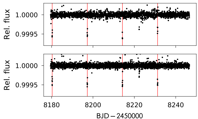
Fig. 2. Detrended K2 light curves of HD 119130 using the two methods described in Section 2. Top panel: Dai et al. (2017) method à la Vanderburg & Johnson (2014). Bottom panel: Pallé et al. (2018) method based on the Everest pipeline (Luger et al. 2018). The vertical red lines mark the position of each detected transit.
