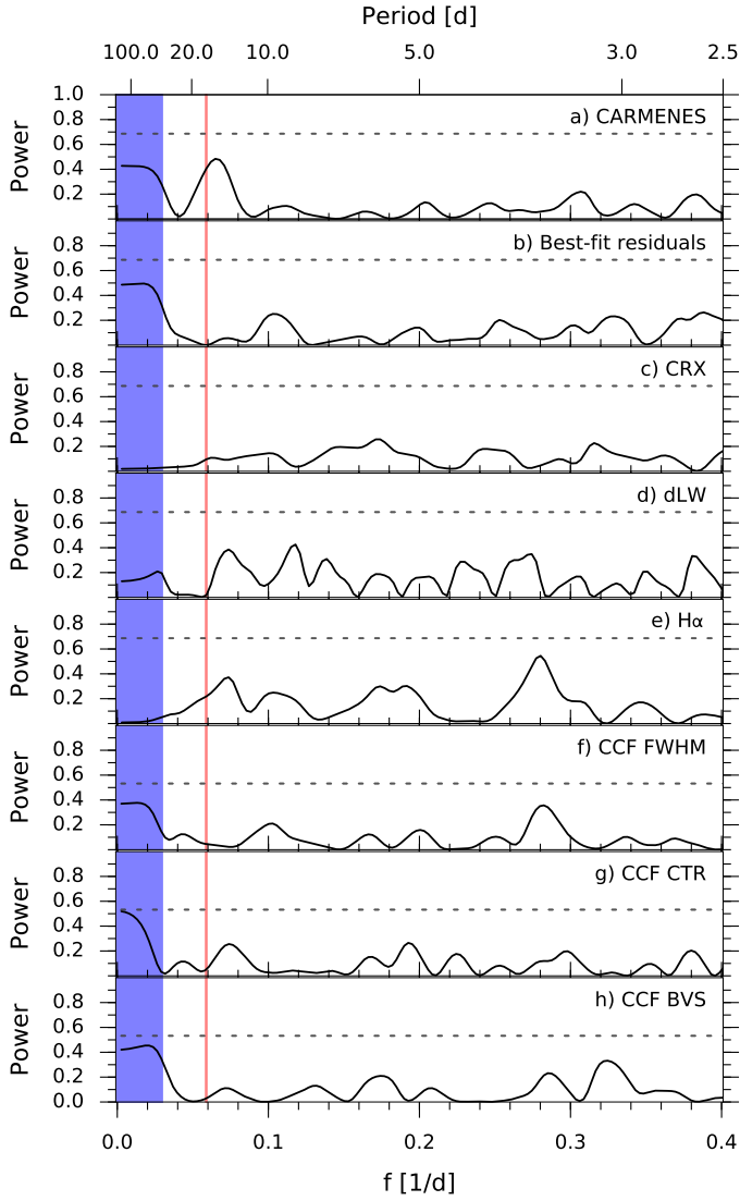
Fig. A.1. GLS periodograms of CARMENES RVs (a) and its residuals (b) after removing the planet signal at f = 0.06 \text{ d}^{-1} derived from K2 photometry, marked in red. Panels (c–e) show periodograms of the chromatic index, differential line width, and H\alpha index, while panels (f–h) show periodograms for the cross-correlation function full-width half-maximum, contrast, and bisector velocity span. The horizontal dashed line shows the theoretical FAP level of 10%. The shaded blue area indicates the period range longer than the timespan of the observations.
