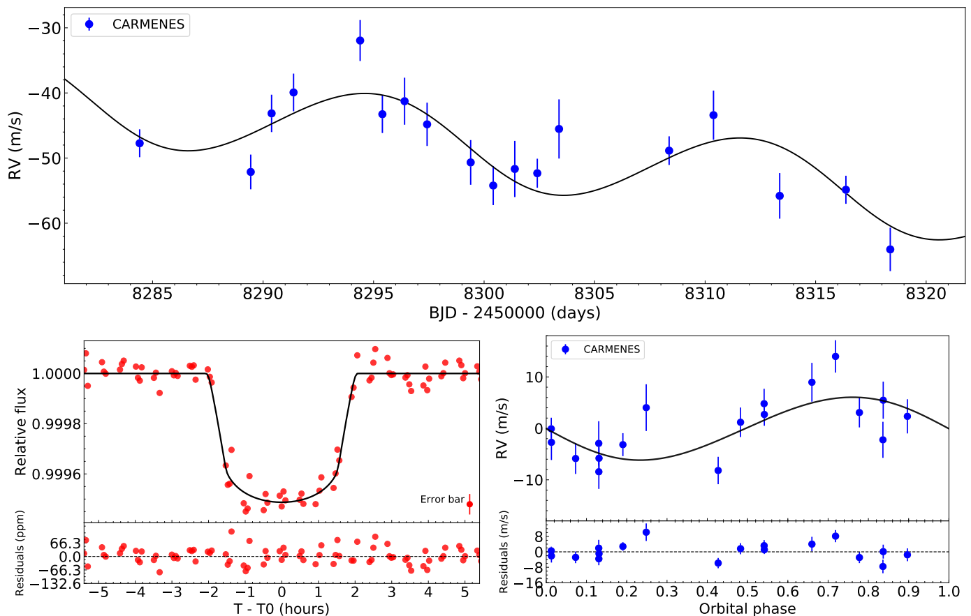
Fig. 5. Top: Time series of CARMENES RVs. Bottom left: Phase-folded K2 light curve to the orbital period of HD 119130 b and residuals. Bottom right: Phase-folded RV curve to the same period and the linear trend subtracted. The solid black line in all panels indicate the preferred best-fit model M1.
