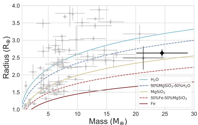
Fig. 6. Mass-radius diagram for all known planets with masses between 0.5–30 M_{\oplus} and radius 1–4 R_{\oplus} determined with a precision better than 30%, comprising from Earth-like to sub-Neptune regimes. HD 119130 b is shown in black, while K2-66 b (Sinukoff et al. 2017) is shown in grey. Data are taken from the TEPICat database of well-characterized planets (Southworth 2011). Theoretical models for the planet’s internal composition are taken from Zeng et al. (2016).
