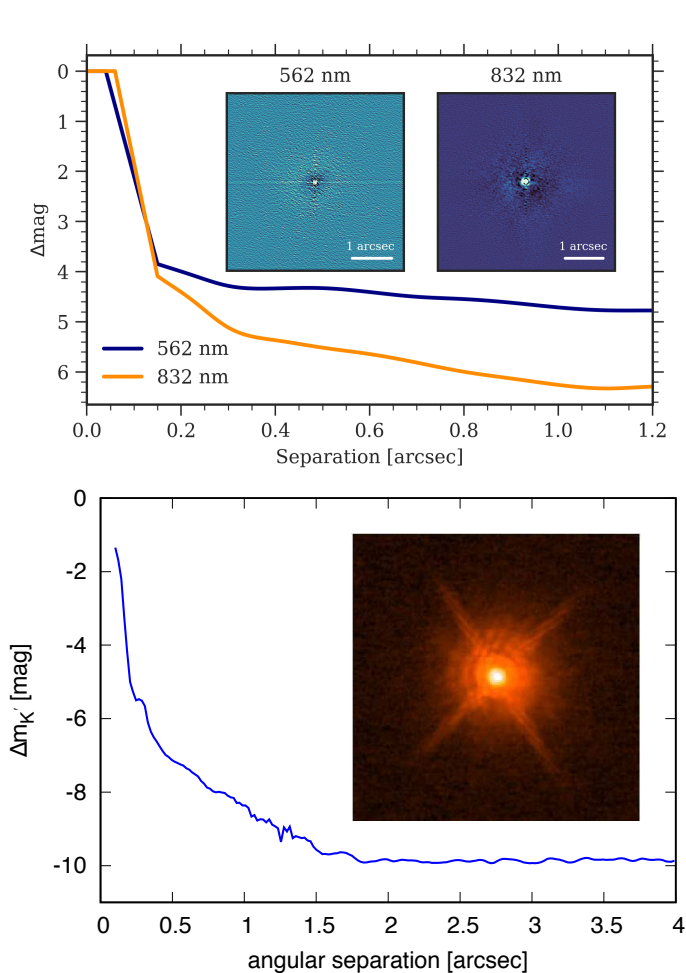
Fig. 3. Top panel: reconstructed images in the 562 nm and 832 nm narrow bands (inset) and their resulting 5\sigma contrast curves from WIYN/NESSI speckle interferometry. Bottom panel: Subaru/IRCS+AO188 combined saturated image and 5\sigma contrast light curve of HD 119130.
