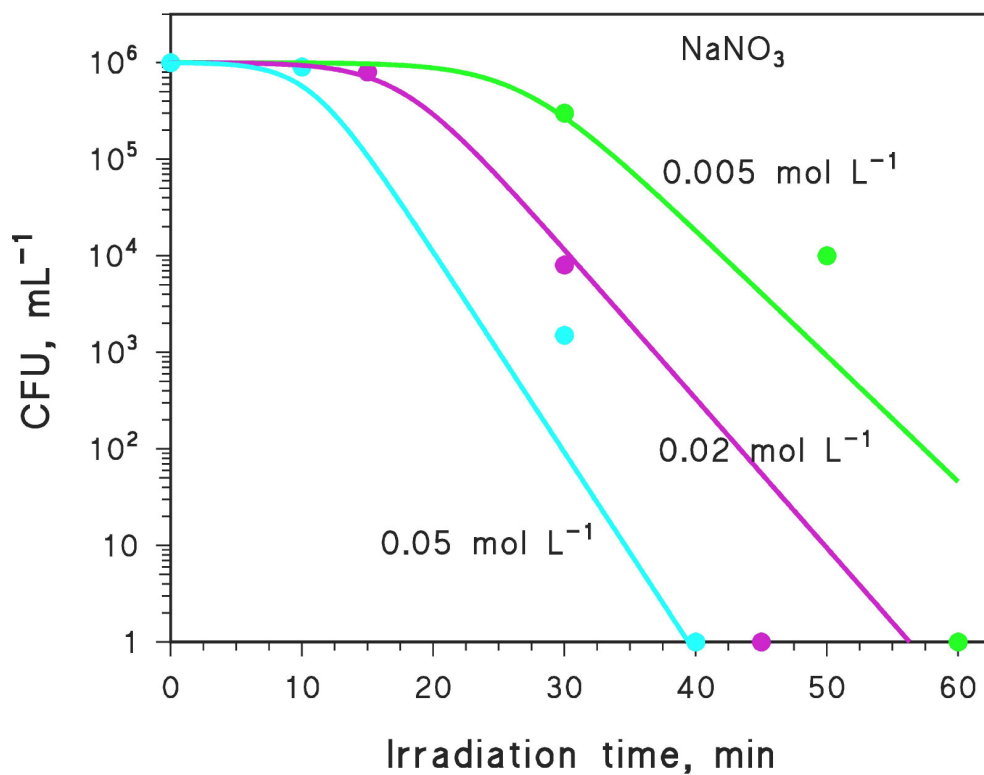
Figure 5. Comparison between the experimental data (solid circles) of bacteria photoinactivation upon UVB irradiation of NaNO 3 (see Figure S4A, with green = 0.005 M NaNO 3 , purple = 0.02 M NaNO 3 , and light blue = 0.05 M NaNO 3 ) and our model predictions (solid curves), based on Eqs. (2-4) in the main text. In particular, it was k_{\text{endo}} = 0.19 \text{ min}^{-1} , L_{\text{endo}} = 34.6 \text{ min} , k_{\text{exo}} = k_{HO^\bullet}^{E.coli} [HO^\bullet] , and L_{\text{exo}} as per Eq. (3) in the main text.
