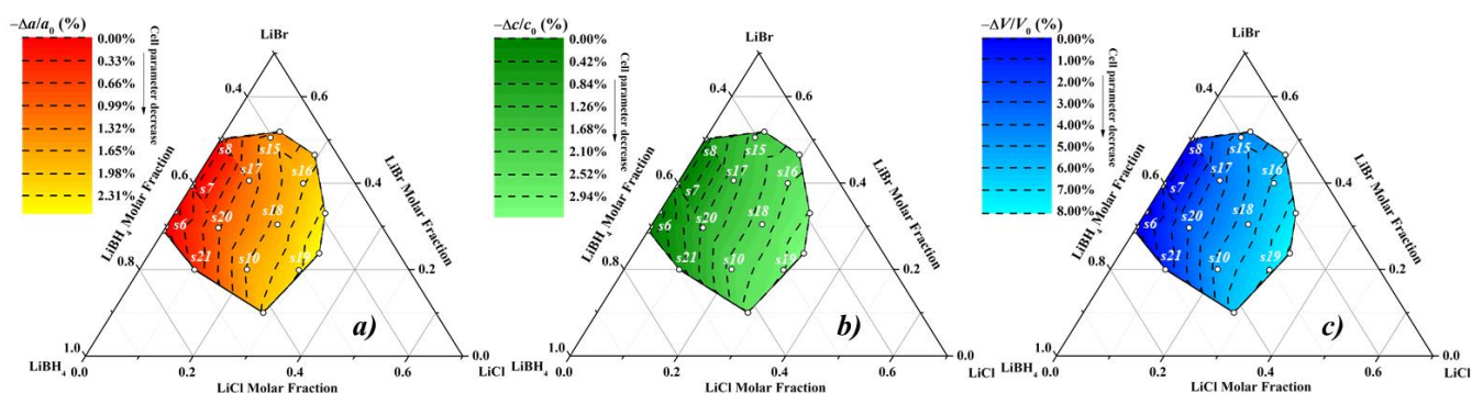
Figure 5. RT maps of (a) -(\Delta a)/a_0 % cell parameter (b) -(\Delta c)/c_0 % c cell parameter and (c) -(\Delta V)/V_0 % volume of the hexagonal solid solution h\text{-Li}(\text{BH}_4)_{1-\alpha-\beta}(\text{Br})_\alpha(\text{Cl})_\beta obtained by Rietveld refinement. a_0 , c_0 and V_0 refer to the parameters of sample s6 taken as a reference. \Delta represents the variation of the cell parameters and volume with respect to the reference values. Dashed lines correspond of the values and lines shown in the legend.
