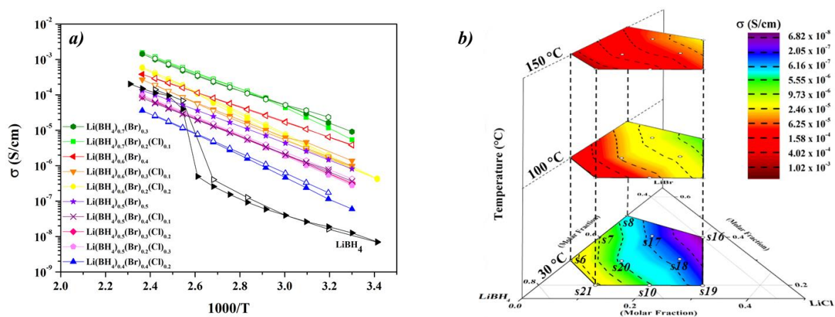
Figure 7. (a) Li-ion conductivity of samples in the hexagonal solid solution in the LiBH 4 -LiBr-LiCl system. Open symbols represent the cooling ramp, close symbols the heating one. b) Contour map of Li-ion conductivity as a function of composition for three selected temperatures. Iso-conductivity dashed lines correspond to the values and lines shown in the legend.
