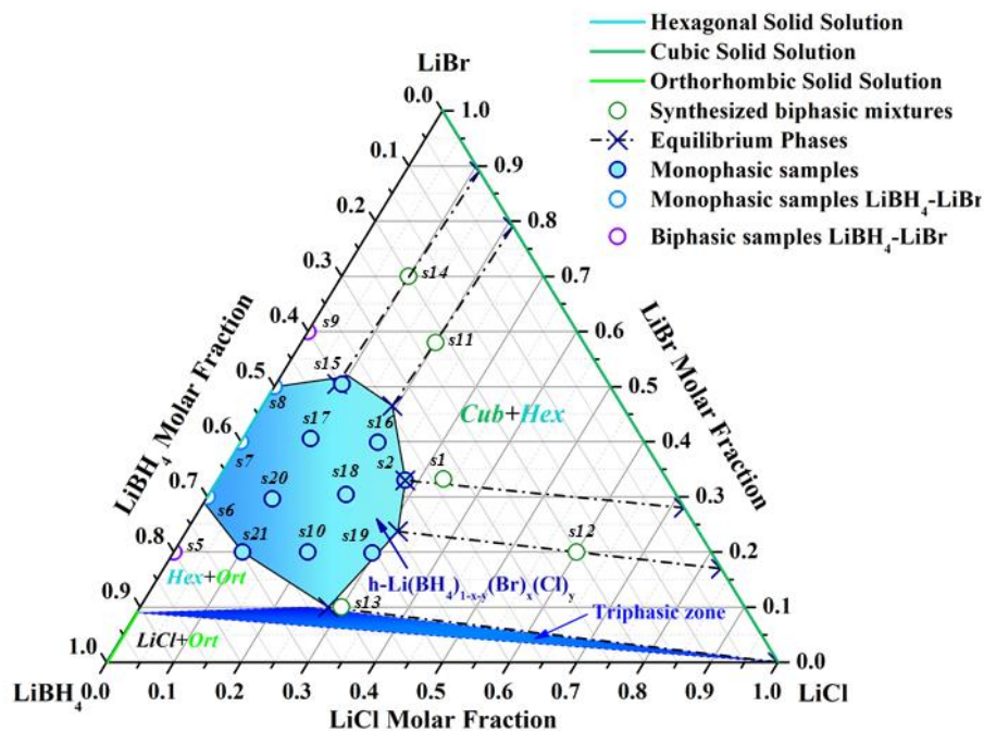
Figure 4. Ternary phase diagram of \text{LiBH}_4\text{-LiBr-LiCl} system at room temperature, obtained by X-ray diffraction analysis. Light filled area is the monophasic zone of hexagonal \text{Li}(\text{BH}_4)_{1-\alpha-\beta}(\text{Br})_\alpha(\text{Cl})_\beta solid solution. Dark filled area indicates a triphasic zone, where \text{Li}(\text{BH}_4)_{0.62}(\text{Br})_{0.1}(\text{Cl})_{0.28} , \text{o-Li}(\text{BH}_4)_{0.9}\text{Br}_{0.1} and pure \text{LiCl} are present. The analysed samples are indicated in the figure and they refer to Table 1.
