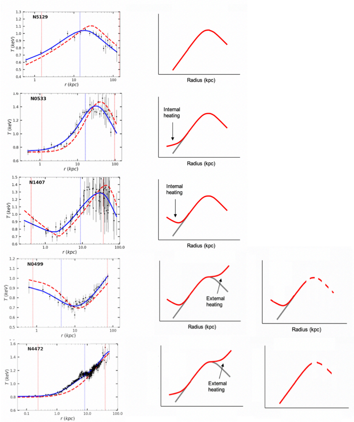
Figure 7. The left-hand panels show examples of hybrid-bump (without a break), hybrid-bump (with an inner break), double-break, hybrid-dip, and positive temperature profiles (top to bottom). The right-hand panels show a graphic illustration of how each profile may be explained by a “universal” profile. The grey curve represents the fiducial profile and the red curve shows the observed profile with deviation from the fiducial profile.
