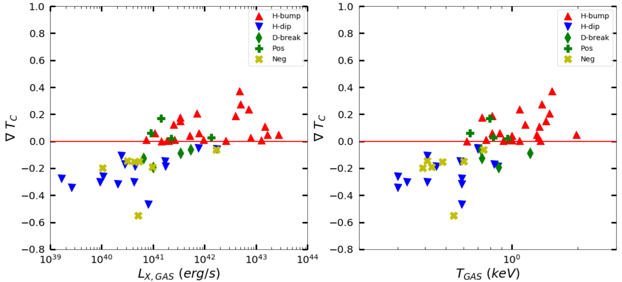
Figure 8. The inner T-gradient ( \nabla T_{\text{CORE}} ) against the temperature ( T_{\text{GAS}} ) and X-ray luminosity ( L_{\text{X,GAS}} ) of the hot gas. All symbols are the same as in Figure 5.
