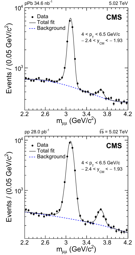
Fig. 1. Dimuon invariant mass distribution showing the J/\psi and \psi(2\text{S}) peaks in pPb (top panel) and pp (bottom panel) data, after applying the \ell_{J/\psi} selection, for -2.4 < y_{\text{CM}} < -1.93 and 4 < p_{\text{T}} < 6.5 \text{ GeV}/c . The fits to the distributions are also shown.
