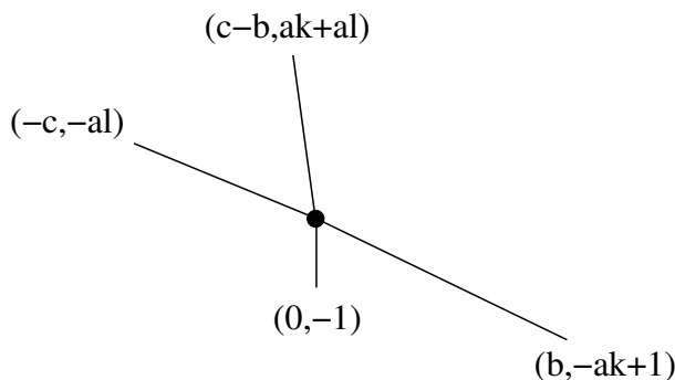
Figure 3: (p,q) -web for the L^{a,b,c} theories.
