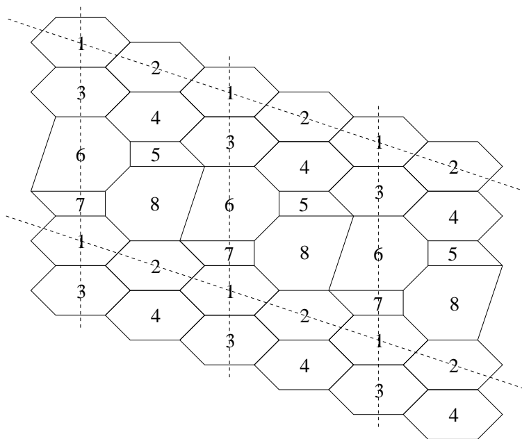
Figure 11: Brane tiling for a Seiberg dual phase of L^{2,6,3} .
