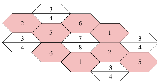
Figure 12: Brane tiling for L^{2,6,4} .
