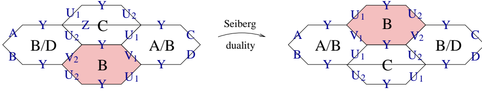
Figure 6: Seiberg duality on a self-dual node that does not change the hexagon content.
