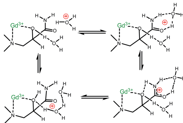
Scheme 2 Mechanism of the H + assisted exchange of –OH and –CONH– protons of Gd(HPADO3A). The free rotation around the C2–C3 \sigma bond of the pendant arm guarantees the same mechanism for both enantiomers at C2.
