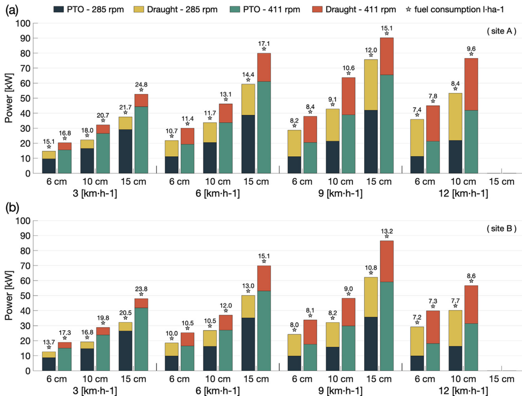
Fig. 8 – Average power [kW] required by the power harrow at different tractor speeds, rotor working depths and rotor speeds for site A (a) and site B (b). Fuel consumption [l ha -1 ] of the tractor is indicated by the numbers above the grey stars.
