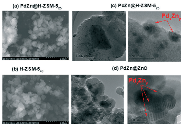
Fig. 3 SEM (a) and (b) and TEM (c) and (d) of the catalyst samples investigated. The PdZn@H-ZSM-5 sample was reduced in H 2 at 500 °C for 4 h, and the PdZn@ZnO sample was pretreated in H 2 at 400 °C for 1 h, prior to the investigation. The Pd x Zn y phases were determined using d-spacing values from the HRTEM see details in the ESI† Fig. S2.
