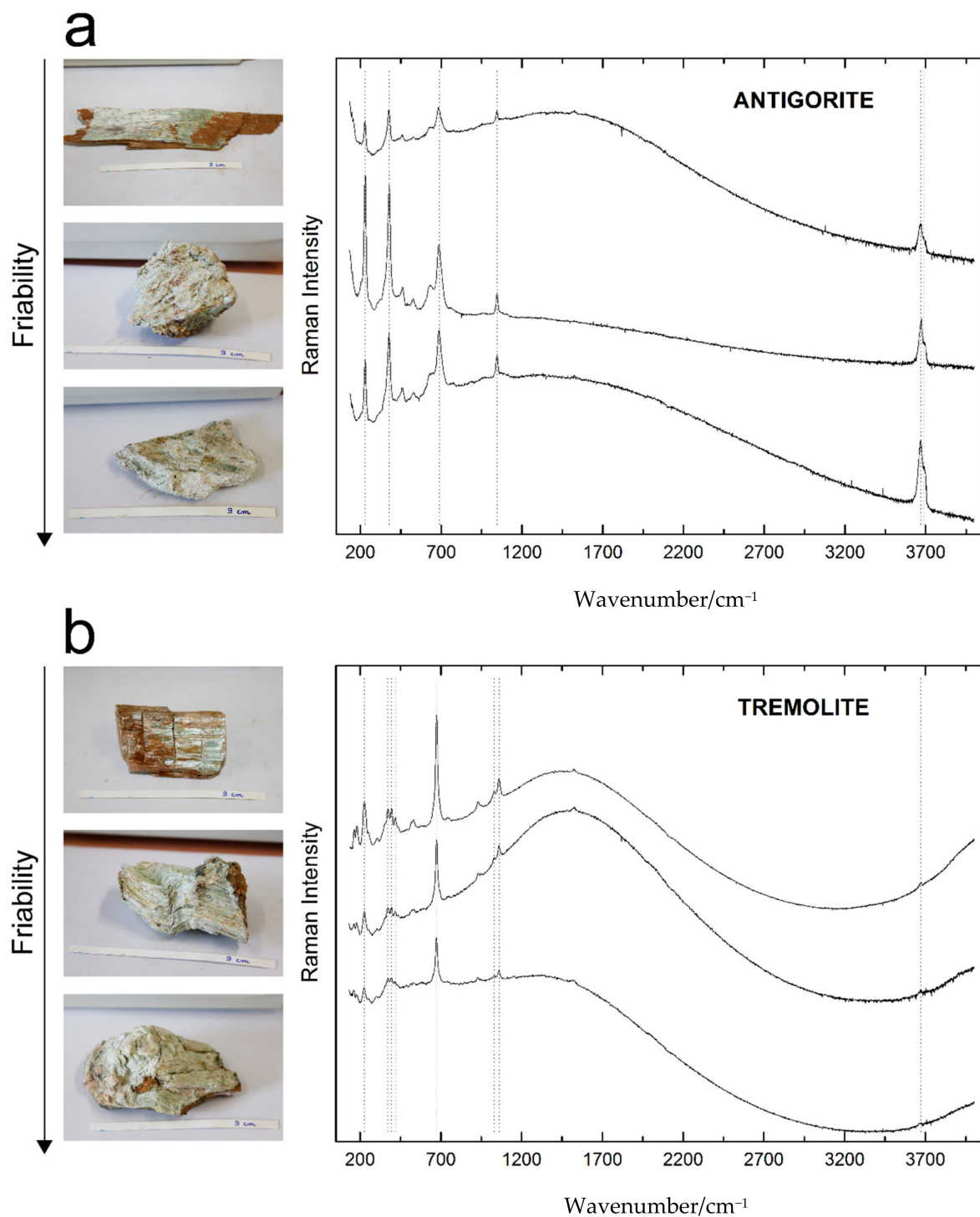
Figure 3. Estimation of performance of portable Raman on differently cohesive, from massive to friable-powdered, asbestos-bearing veins from Tontouta Ni- open pit mine. (a) antigorite; (b) tremolite. Raman spectra were acquired in the extended spectral region (100–4000 cm -1 ).
