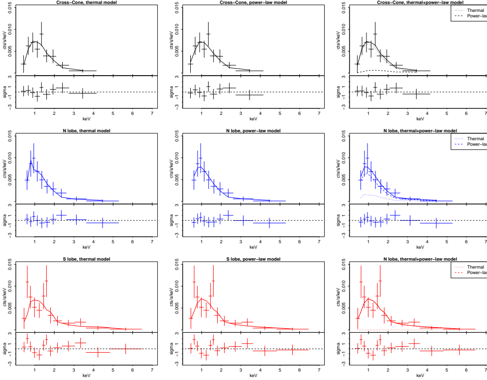
Fig. 8. Spectral fits in the 0.3 – 7 keV band performed with a thermal xspecc (left column), power-law (central column) and mixed thermal+power-law (right column) models. From top to bottom we show spectra extracted in the cross cone, N lobe, and S lobe regions. In upper portion of each panel the full line represents the best fit model and the crosses represent the data points, while in lower portion of each panel is presented the residual distribution. For the thermal+power-law model (right column) the dotted line represents the thermal component, the dashed line represents the power-law component, and the full line represents the total model.
