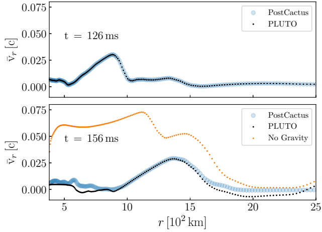
Figure D2. Radial profiles of the angle-averaged radial velocity at 126 ms and 156 ms after merger (upper and lower panels, respectively). The blue dots are obtained by importing data from our reference BNS merger simulation at the given time (Section 2.1). The black dots correspond instead to the result of our test PLUTO simulation, which starts from the same initial data at 126 ms and then evolves the system according to the adopted prescriptions (see text for details). Finally, the orange dots correspond the same PLUTO simulation where we neglect the contribution of gravity.
