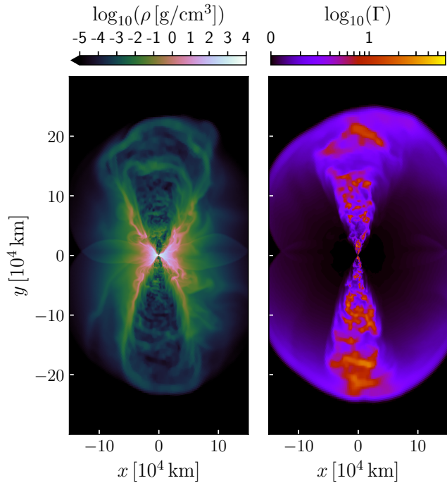
Figure 12. Meridional view of rest-mass density (left) and Lorentz factor (right) at 1112 ms after merger for the case with remnant NS collapse at 201 ms. The spatial and color scales used here are the same adopted in Figure 6.
