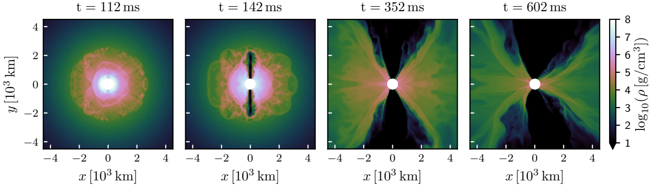
Figure 3. Meridional view of the rest-mass density at different times for our fiducial model (see Section 3.1). Left panel refers to the initial jet launching time. As in Figure 1, the white circle of 380 km radius corresponds to the excised region.
