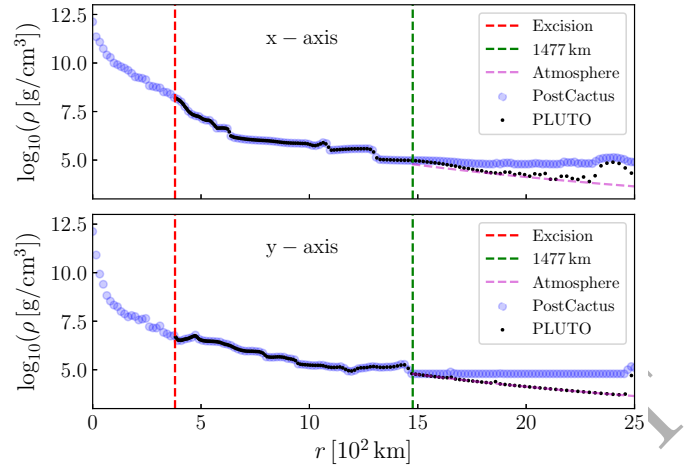
Figure 2. Radial profile of the rest-mass density along the x - and y -axes for data imported from the reference BNS merger simulation at 101 ms post-merger. The blue and black dots refer to the result of the PostCactus interpolation and to the final setup in PLUTO, respectively. The vertical red- and green-dashed lines indicate, respectively, the excision radius and the radial distance (1477 km) above which we replace the uniform artificial density floor with a profile decaying as r^{-5} (shown with a magenta-dashed line). See text for further details.
