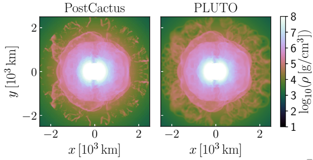
Figure D3. Meridional view of the rest-mass density at 156 ms after merger for the same two cases shown in Figure D2, i.e. data imported from our reference BNS merger simulation (left) and the result of the evolution in PLUTO starting from data imported at 126 ms (right). The white circle of 380 km radius corresponds to the excised region (as in Figs. 1 and 3).
