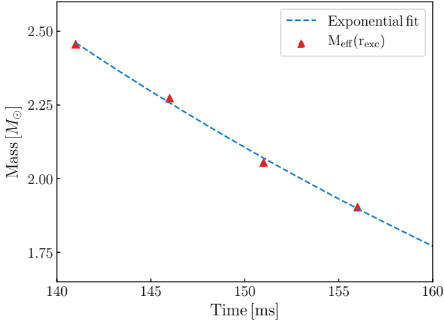
Figure 11. Evolution of the effective mass at the excision radius (380 km) at times \geq 141 ms after merger. Red triangles are the values of M_{\text{eff}}(r_{\text{exc}}) extracted from the BNS merger simulation, while the dashed blue curve corresponds to an exponential fit (see text).
