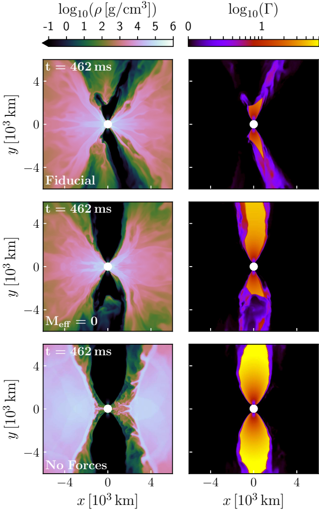
Figure 5. Meridional view of rest-mass density (left) and Lorentz factor (right) at 462 ms after merger. Top, central, and bottom rows refer to the fiducial simulation (Sect. 3.1), the one with M_{\text{eff}}=0 (see Sect. 2.2), and the one without external forces (Sect. 3.2), respectively.
