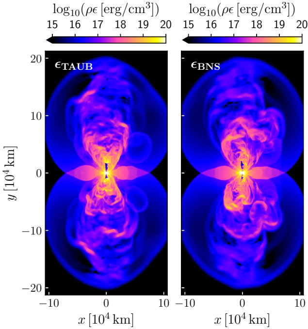
Figure B1. Meridional view of internal energy density at 762 ms after merger. Left panel refers to our fiducial model, where the initial rest-mass density and pressure are directly imported from the reference BNS merger simulation, while the specific internal energy \epsilon is derived via the Taub EOS. For the case on the right, the imported quantities are instead rest-mass density and \epsilon , while the quantity derived via the Taub EOS is the pressure.
