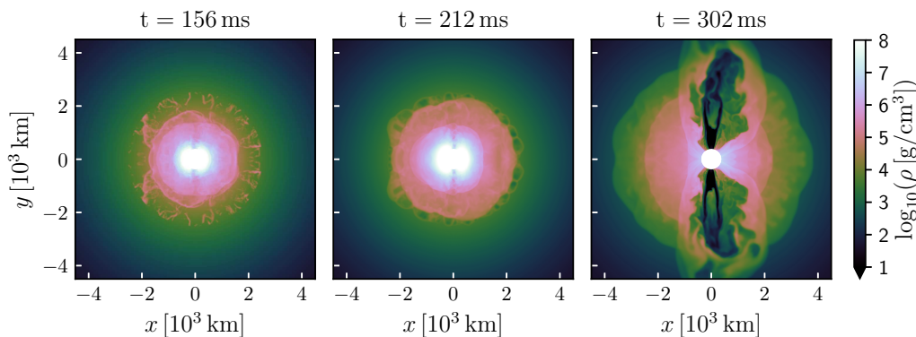
Figure 10. Same as Figure 3 for the model with collapse at 201 ms (and jet launching at 212 ms).
