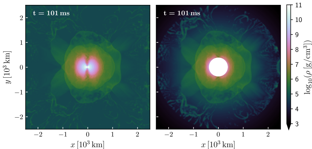
Figure 1. Meridional view of the rest-mass density as obtained by importing data from the reference BNS merger simulation at 101 ms post-merger (see text). The left panel shows the result of the PostCactus interpolation, while the right panel shows the final setup on the PLUTO grid. The white circle of 380 km radius in the right panel corresponds to the excised region (that we do not evolve in PLUTO).
