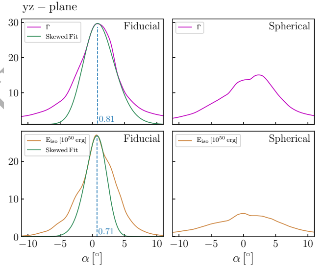
Figure 9. Same as Figure 8 for the yz -plane. In this case, the sign of \alpha corresponds to the sign of z .
