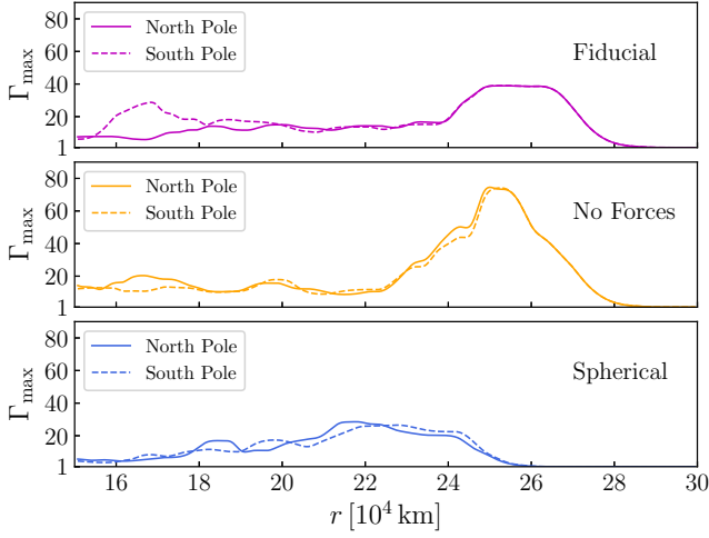
Figure 7. Radial profiles of maximum Lorentz factor at 1012 ms after merger (maximum value achieved at each radial distance). North and south profiles are shown for the same three cases of Figure 6: our fiducial simulation (top), the one without external forces (center), and the one with simplified isotropic surrounding environment (bottom).
