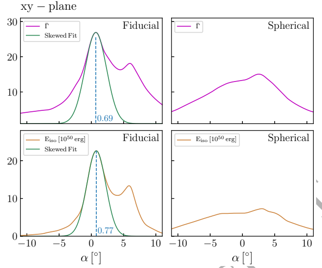
Figure 8. Angular profiles (north side only) on the xy -plane of the radial-averaged Lorentz factor (top) and isotropic-equivalent energy E_{\text{iso}} (bottom) at the jet’s head (see text for details) and at 1012 ms after merger. Left panels refer to our fiducial simulation, while right panels refer to the one with simplified isotropic surrounding environment (Section 3.3). Here, \alpha is the angle with respect to the injection axis (i.e. the y -axis), with positive/negative sign for positive/negative x . The green curve in the left panels corresponds to the skewed function that best-fits the central peak of the profile. The vertical dashed blue line marks the angular position of the peak.
