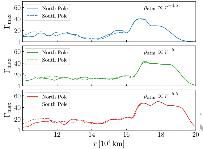
Figure A1. Same as Figure 6 for our fiducial model with different power-law exponents for the radial profile of density and pressure in the atmosphere, at 762 ms after merger.
