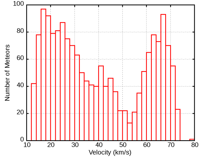
Fig. 11. Histogram of sporadic fireball entry velocities. Two populations can be observed: 1) low speed objects corresponding mostly to asteroidal orbits, 2) fast objects corresponding to TNOs or comet-like objects. this dichotomy has also been observed by Drolshagen et al. (2014) with the CILBO network for smaller objects.
