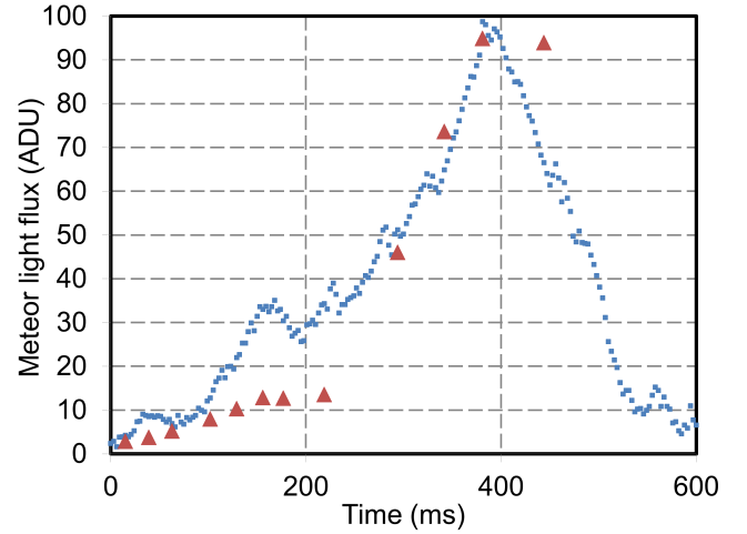
Fig. 14. Raw light flux from a bolide observed on 14 August 2019 at 03h07m02s UTC. Red triangles: Dijon FRIPON camera data (30 Hz, 12bits). Blue squares: radiometer prototype data (20 kHz, 14 bits). The faster acquisition rate and the higher amplitude dynamic range of the radiometer allows more detailed observations of the meteor fragmentation and of high speed luminosity variations.
