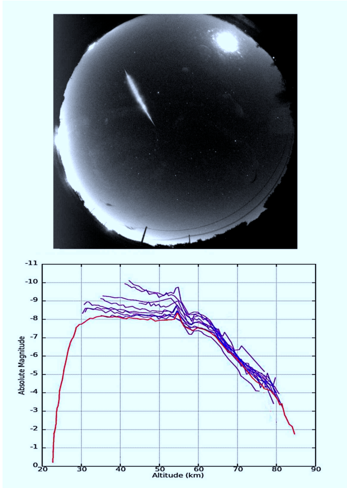
Fig. 5. Top: 27 February 2019 event seen by Beaumont-lès-Valence FRIPON camera; Bottom: absolute magnitude light-curves of the event as seen by 15 cameras, red curve is Beaumont-lès-Valence. It is clear that the saturation limit is around magnitude -8 (all the other light-curves fall above this limit). Cameras located further away may be able to measure more non saturated data, but all the cameras do become heavily saturated as the bolide reaches its maximum luminosity.
