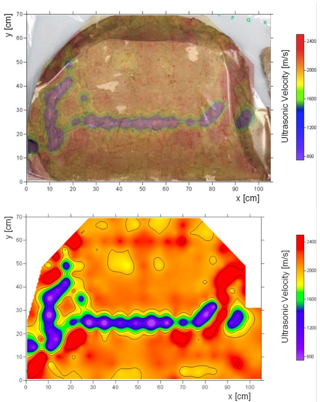
Figure 8. The images show the velocity trends of the ultrasounds in the limestone.
