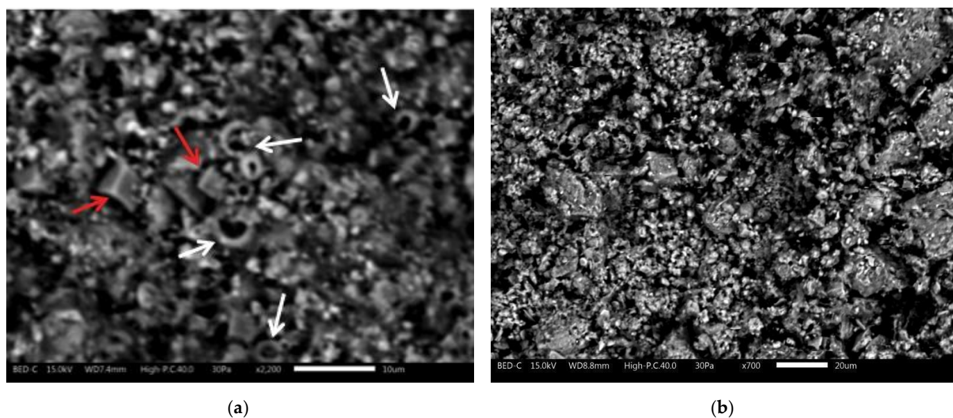
Figure 5. Electron microscope image (SEM backscattered electrons) of: (a) sample 1, the fine grain size of the micrite crystals is clearly visible; white arrows: micropaleontological content (coccoliths); red arrows: dolomite crystals; (b) sample 2, microscopic aspect: micritic crystals and euhedral crystals.
