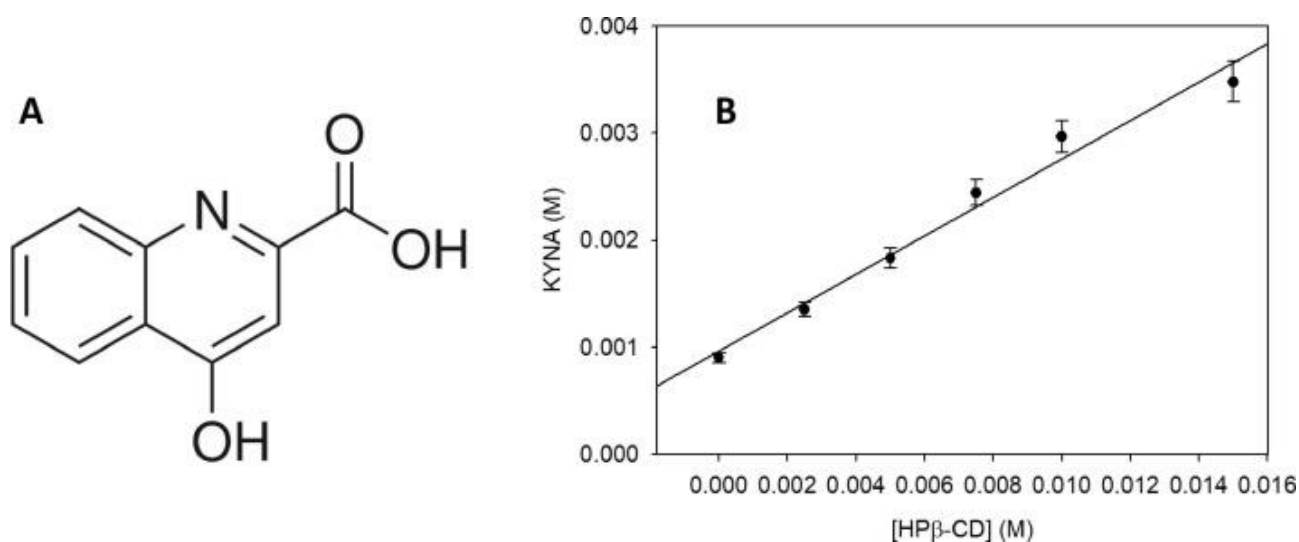
Fig. 1. (A) Structure of KYNA. (B) Higuchi and Connors plot, Effect of HPβ-CD on KYNA solubility (25 °C in water).
