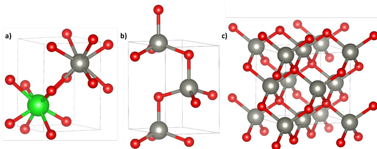
Figure 7. Structures used as input geometries in Zn K-edge EXAFS fits for ZrZn-15. Unit cell of a) tetragonal \text{ZrO}_2 (space group P4 2 nmc; lattice parameters a = 3.60 \text{ \AA} and c = 5.10 \text{ \AA} 33 from Table S1) substituted with Zn; b) h- \text{ZnO} (P6 3 mc; a = 3.25 \text{ \AA} and c = 5.21 \text{ \AA} 35 ) and c) c- \text{ZnO} (F-43m, a = 4.63 \text{ \AA} 36 ). Zinc (grey), Zirconium (green) and Oxygen (red) atoms are represented by coloured spheres. Oxygen partial occupancy in model a) is represented by non-filled colours.
