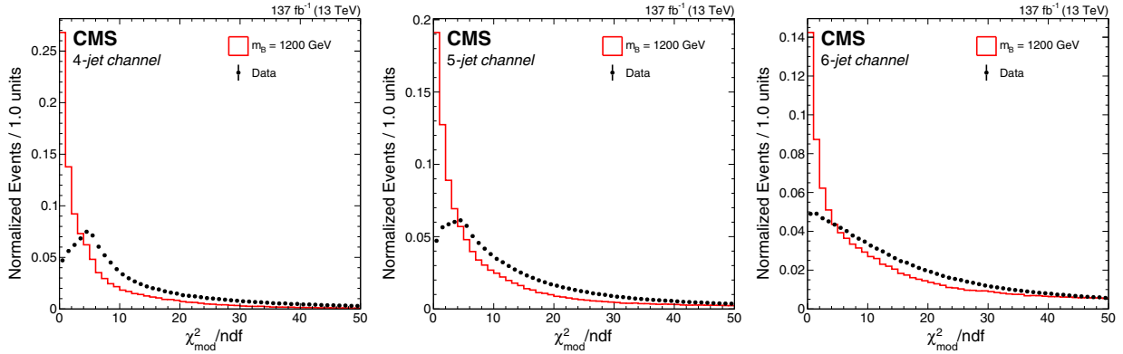
FIG. 3. Distribution of \chi_{\text{mod}}^2/\text{ndf} for the best jet combination for simulated 1200 GeV VLQ events (red histogram) and data (black points), for 4-jet (left), 5-jet (center), and 6-jet events (right). The simulated signal events and data events are normalized to the same integral value within the displayed \chi_{\text{mod}}^2 range.
