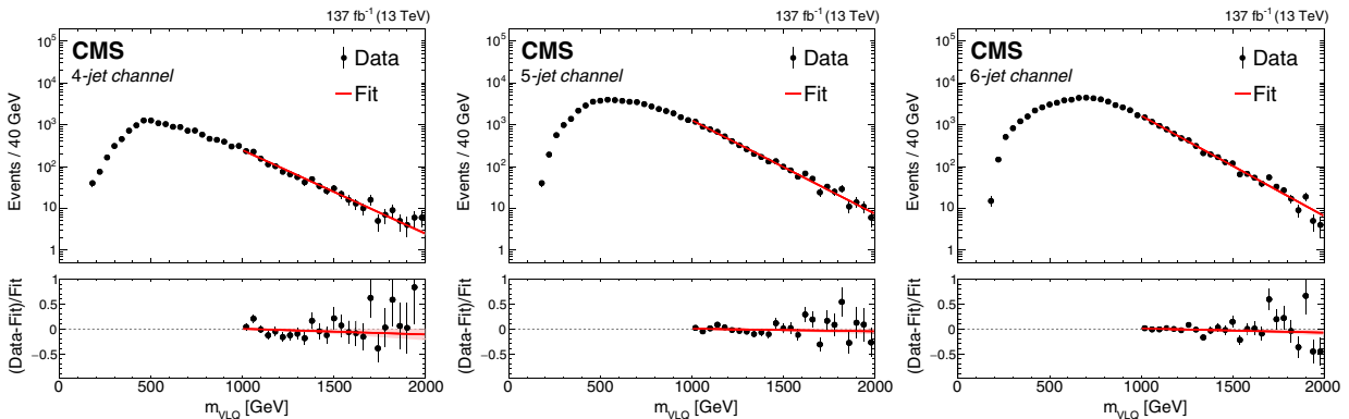
FIG. 4. Distributions of m_{\text{VLQ}} for the jet combination with the lowest \chi_{\text{mod}}^2 in 4-jet (left), 5-jet (center), and 6-jet (right) multiplicity events. The red lines show the exponential fit in the range 1000–2000 GeV. The lower panels show the fractional difference, (\text{data} - \text{fit})/\text{fit} .
