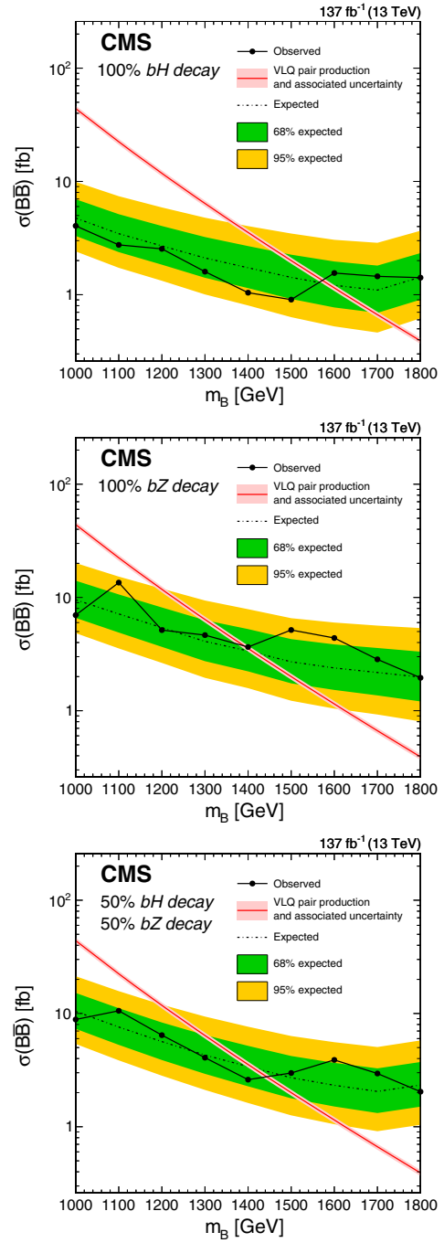
FIG. 11. The 95% confidence limit on the cross section for VLQ pair production as a function of VLQ mass for three branching fraction hypotheses: B(B \rightarrow bH) = 100\% (upper left), B(B \rightarrow bZ) = 100\% (middle), and B(B \rightarrow bH) = B(B \rightarrow bZ) = 50\% (lower). The solid black line indicates the observed limit and the dashed line indicates the expected limit with 1 sigma (green band) and 2 sigma (yellow band) uncertainties. The theoretical cross section and its uncertainty are shown as the red line and pale red band; the band is only slightly visible outside the line.
