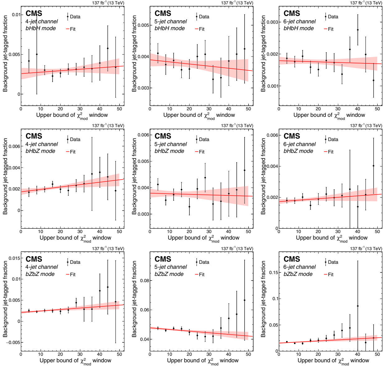
FIG. 6. Dependence of the BJTF on \chi_{\text{mod}}^2/\text{ndf} in the low-mass (500–800 GeV) VLQ region, for 4-jet (left column), 5-jet (center column), and 6-jet (right column) multiplicities, and for the bHbH (upper row), bHbZ (middle row), and bZbZ (lower row) event modes. The data are shown as black points with vertical error bars, and the linear fit and associated uncertainty are shown as a solid red line and the shaded red band.
