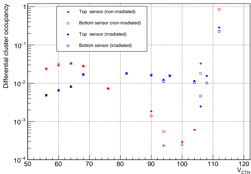
Figure 15. Differential cluster occupancy for non-irradiated and irradiated sensors as a function of V_{\text{CTH}} . A bias voltage of 250 V (600 V) was applied to the non-irradiated (irradiated) mini-module.
