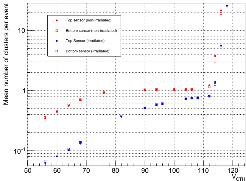
Figure 14. Average number of clusters per event for non-irradiated and irradiated sensors as a function of V_{\text{CTH}} . A bias voltage of 250 V (600 V) was applied to the non-irradiated (irradiated) mini-module.
